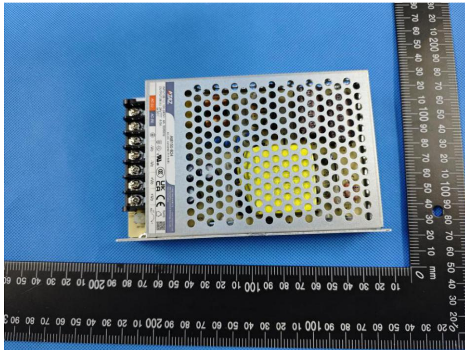
Built-in power supply 2: AM150-B24
