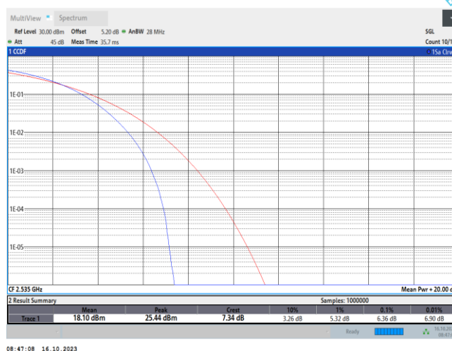
7-7-20MHz-20MHz-QPSK-QPSK-21001-21199-100RB#0-100RB#0
