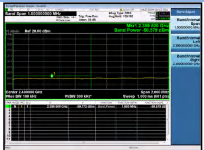
802.11VHT-40 MHz CHANNEL 4, Reference level
