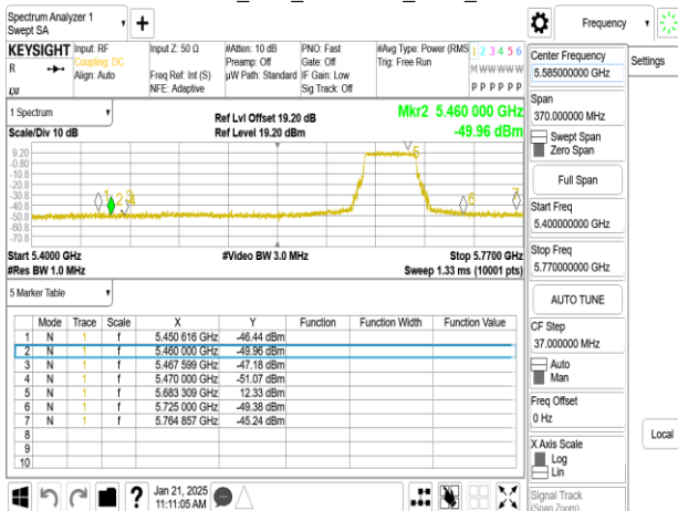
802.11be_40M_5670 MHz_Peak_chain0
