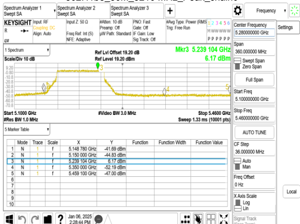
802.11be_80M_5210 MHz_Peak_chain1
