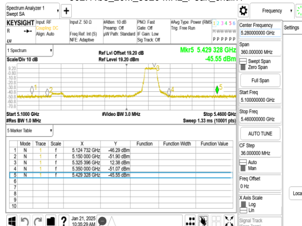
802.11be_20M_5320 MHz_Avg_chain0
