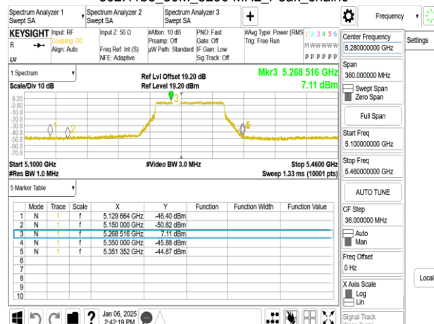
802.11be_80M_5290 MHz_Peak_chain1
