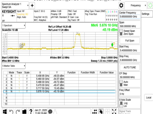
802.11be_20M_5720 MHz_Peak_chain1
