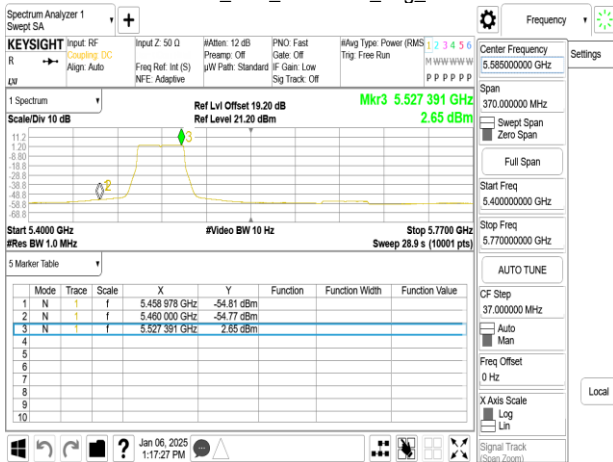
802.11be_40M_5510 MHz_Avg_chain1
