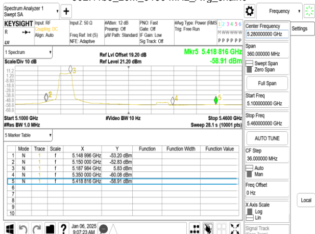
802.11be_20M_5180 MHz_Avg_chain1
