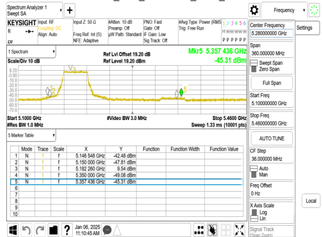
802.11be_40M_5190 MHz_Avg_chain0
