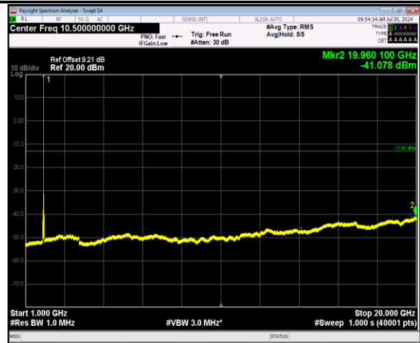
2-2-5MHz-20MHz-64QAM-64QAM-18808-18925-1RB#24-0 RB#0-1000~20000MHz-PASS
