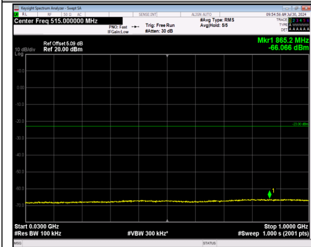
2-2-5MHz-20MHz-64QAM-64QAM-18808-18925-1RB#0- 1RB#99-30~1000MHz-PASS
