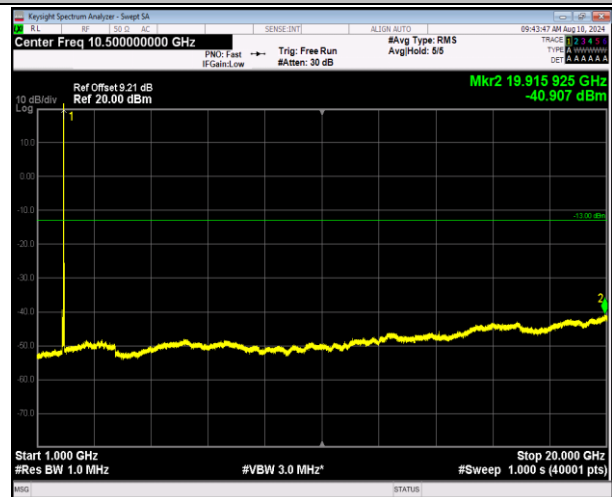
2-2-5MHz-20MHz-QPSK-QPSK-18983-19100-1RB#0-0RB# 0-1000~20000MHz-PASS
