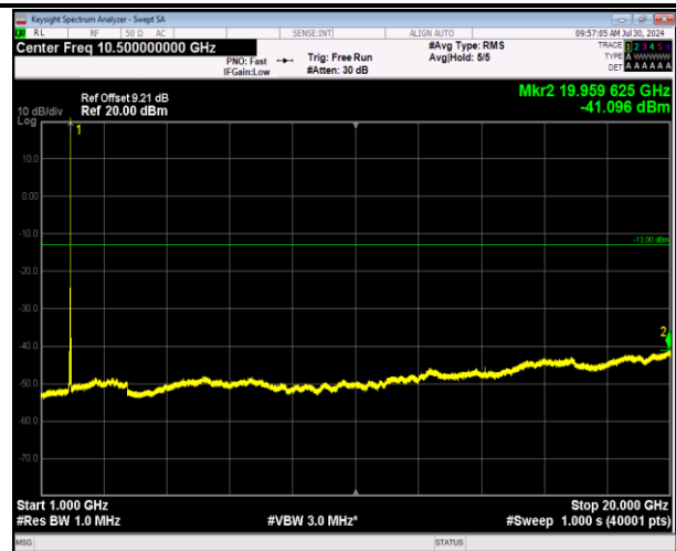
2-2-5MHz-20MHz-64QAM-64QAM-18983-19100-1RB#24-0 RB#0-1000~20000MHz-PASS
