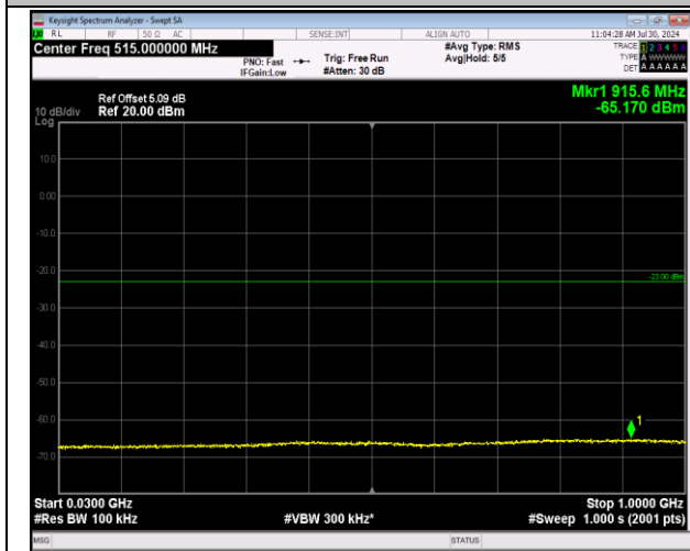
2-2-20MHz-20MHz-64QAM-64QAM-18700-18898-1RB#0 -0RB#0-30~1000MHz-PASS
