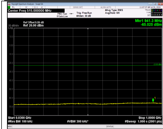
2-2-20MHz-20MHz-64QAM-64QAM-18801-18999-1RB#9 9-ORB#0-30~1000MHz-PASS
