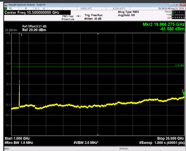
2-2-5MHz-20MHz-16QAM-16QAM-18808-18925-1RB#0-0RB#0-1000~20000MHz-PASS
