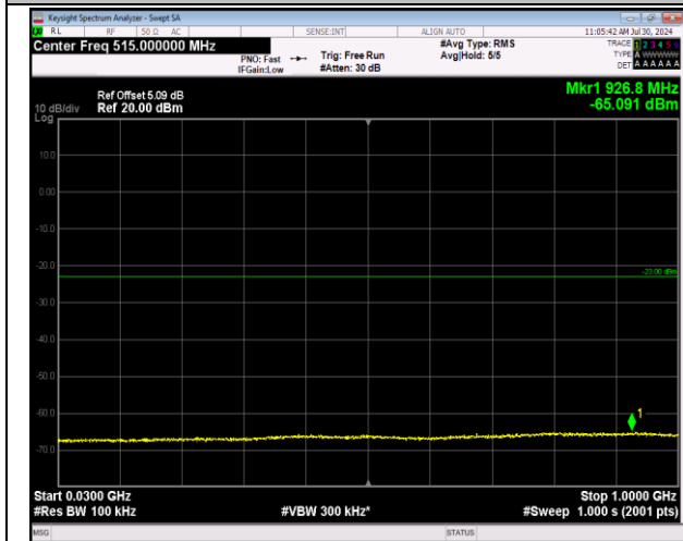
2-2-20MHz-20MHz-64QAM-64QAM-18700-18898-1RB#0 -1RB#99-30~1000MHz-PASS
