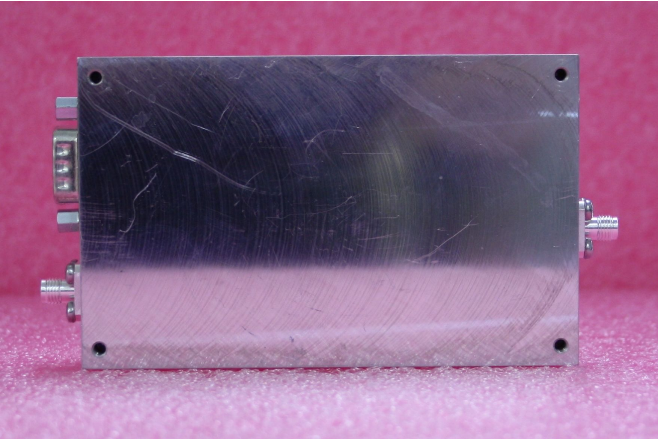
12-030301 380-500MHz 1W 33dB GAIN 12V AMP
