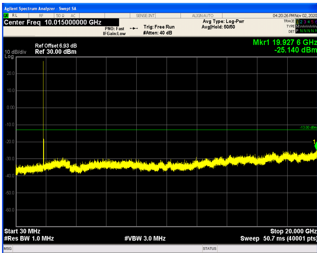
LTE Band2 QPSK BW=20MHz Channel=18700 RB Size=100 Position=#0
