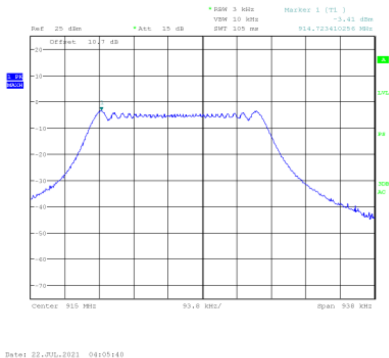
Figure 20 – Mid Channel Power Spectral Density (LoRa)
