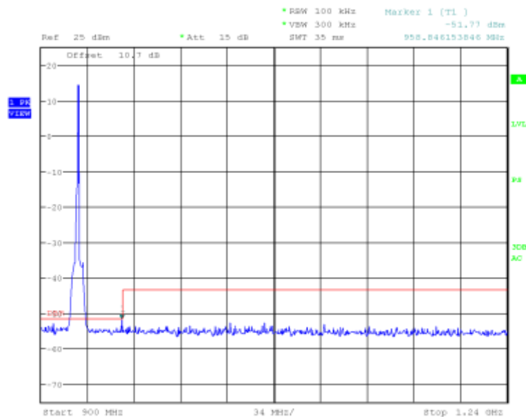
Figure 31 – Low Channel Conducted Band Edge (LoRa, Modulated TX)
