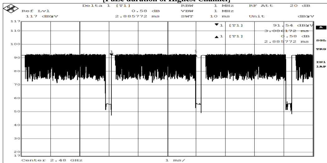
Fig. C [Pulse duration of Highest Channel]
