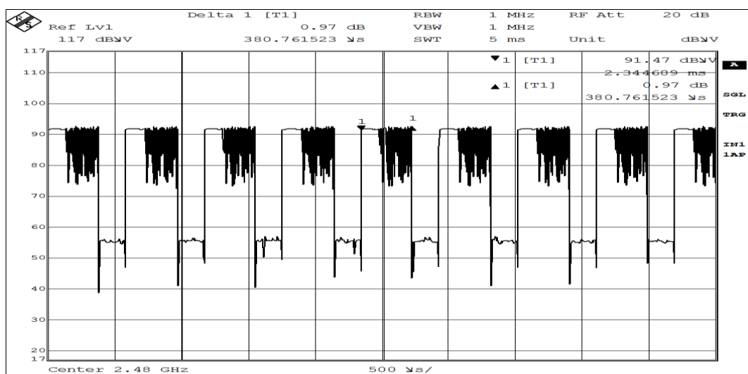
Fig. I [Pulse duration of Highest Channel]
