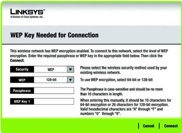
Figure 4-11: WEP Key Needed for Connection
