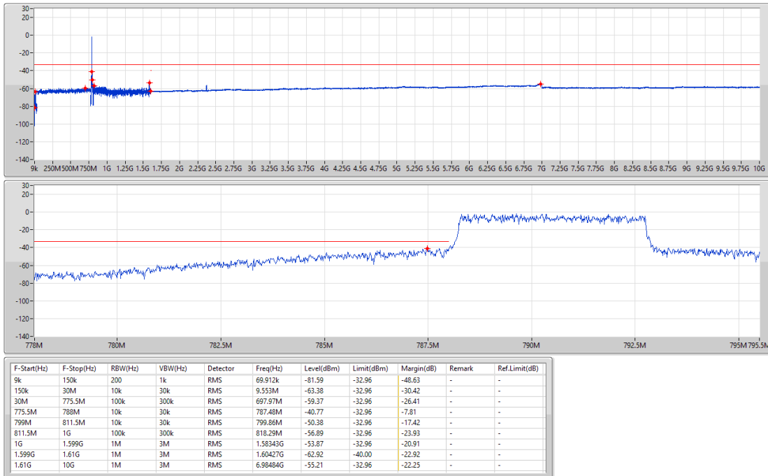
Band 14 LTE_5MHz_Nss1,64QAM_1TX 790.5MHz_64QAM_RB 25,#RB 0
