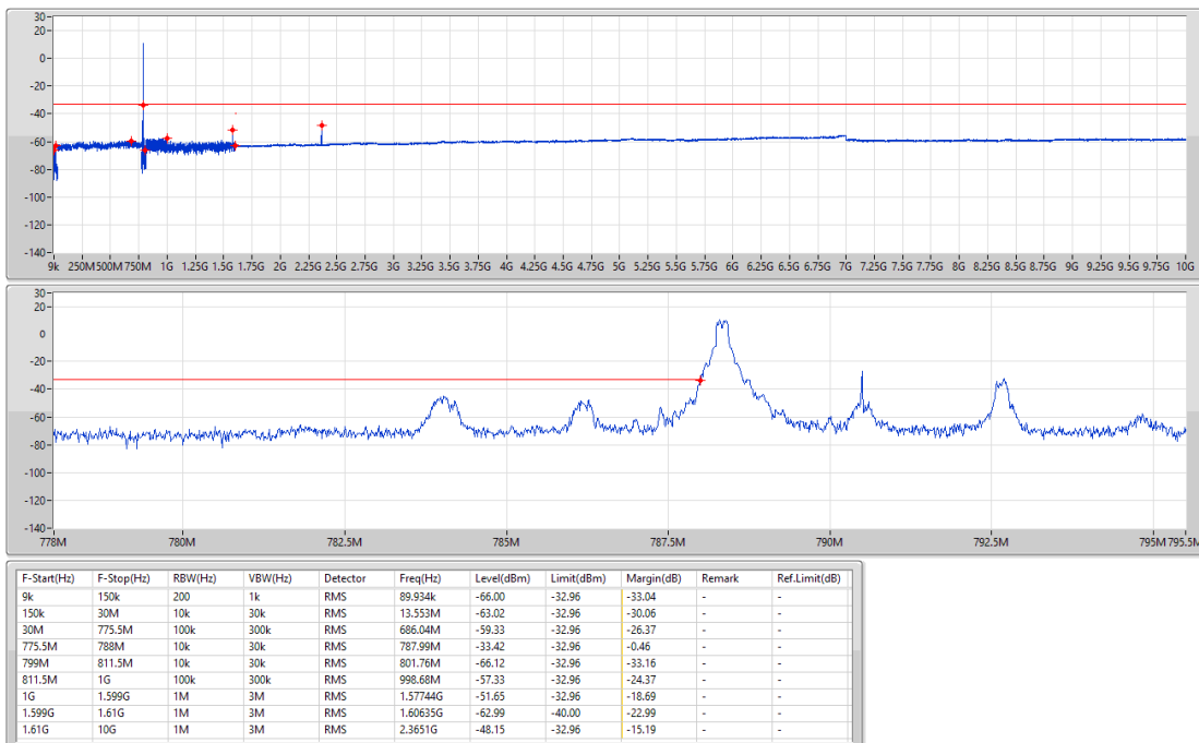
Band 14 LTE_5MHz_Nss1,64QAM_1TX 790.5MHz_64QAM_RB 1,#RB L
