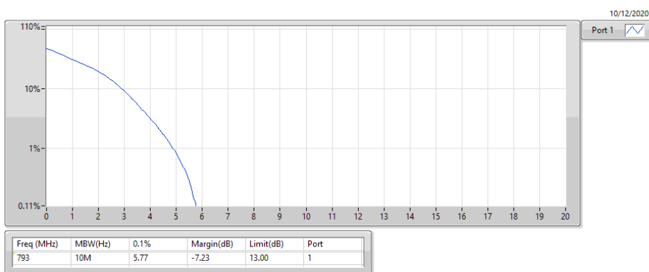
Band 14_LTE_10MHz_Nss1,16QAM_1TX 793MHz_16QAM_RB 50,#RB 0
