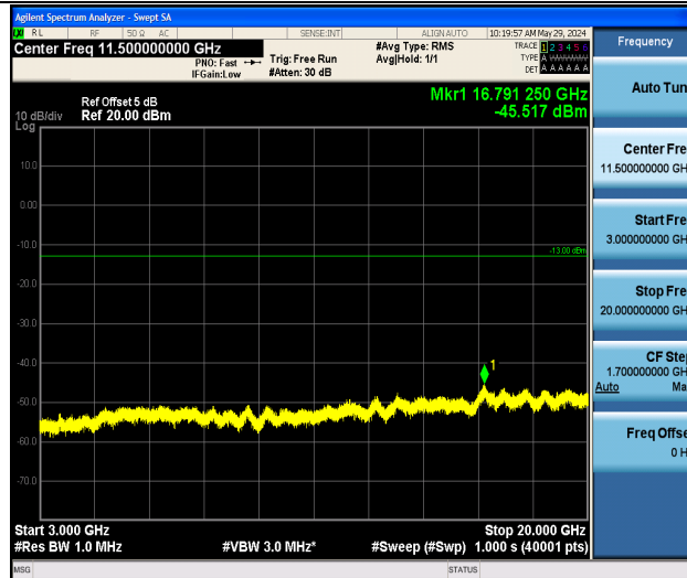
Band2_1.4MHz_QPSK_19193_1RB#0_3000~20000_3000~20000
