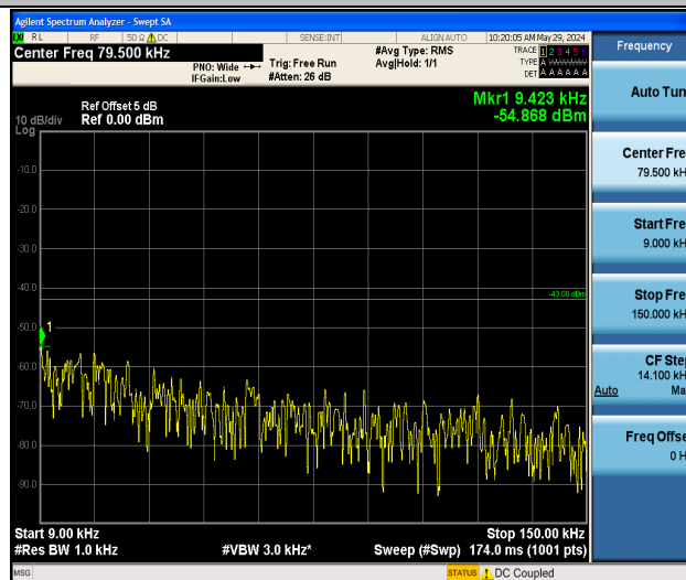
Band2_1.4MHz_16QAM_19193_1RB#0_0.009~0.15_0.009~0.15
