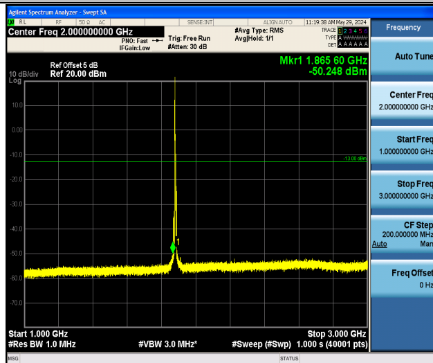
Band2_5MHz_QPSK_18900_1RB#0_1000~3000_1000~3000
