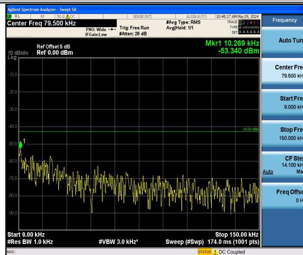
Band2_3MHz_QPSK_18900_1RB#0_0.009~0.15_0.009~0.15
