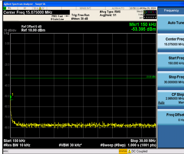
Band2_3MHz_QPSK_19185_1RB#0_0.15~30_0.15~30
