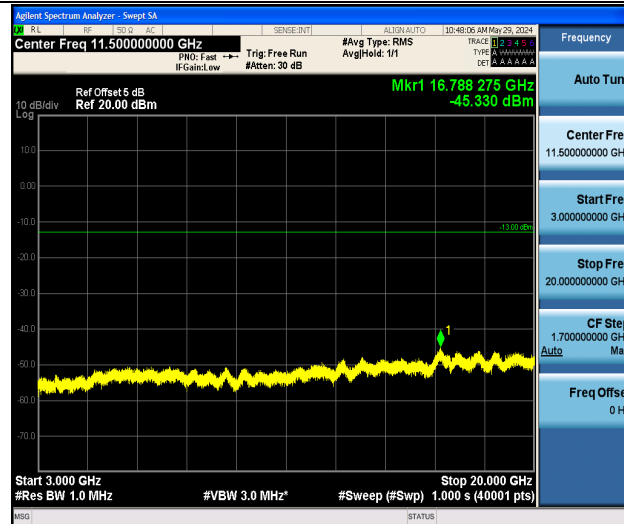
Band2_3MHz_16QAM_18615_1RB#0_3000~20000_3000~20000
