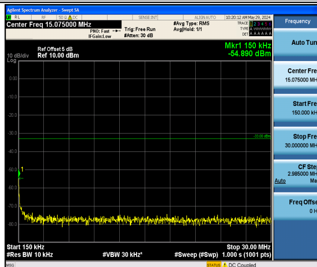
Band2_1.4MHz_16QAM_19193_1RB#0_0.15~30_0.15~30
