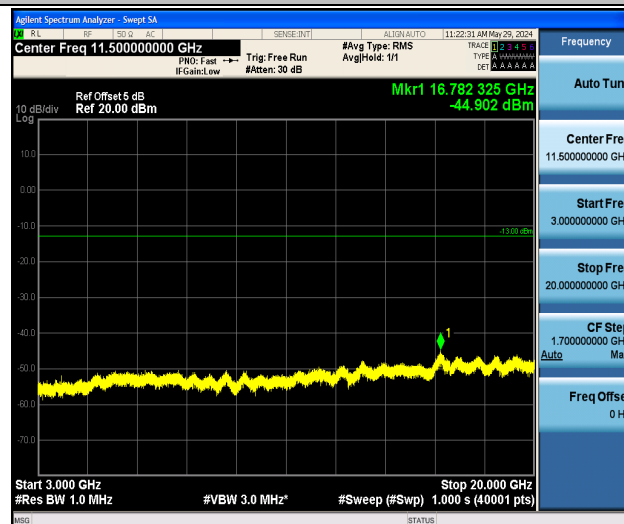
Band2_5MHz_16QAM_19175_1RB#0_3000~20000_3000~20000
