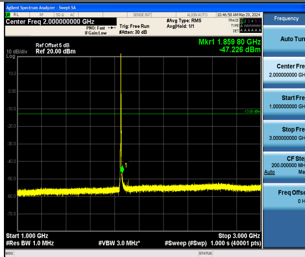
Band2_3MHz_QPSK_18615_1RB#0_1000~3000_1000~3000
