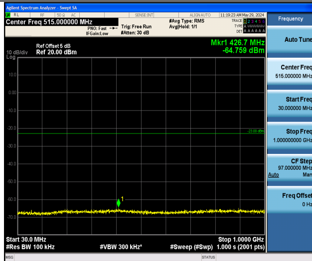
Band2_5MHz_QPSK_18900_1RB#0_30~1000_30~1000
