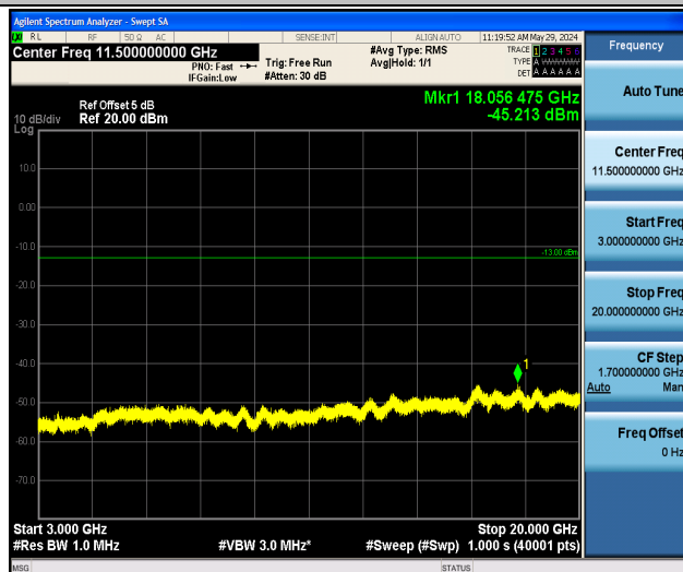
Band2_5MHz_QPSK_18900_1RB#0_3000~20000_3000~20000
