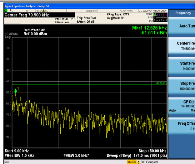
Band2_5MHz_QPSK_18900_1RB#0_0.009~0.15_0.009~0.15
