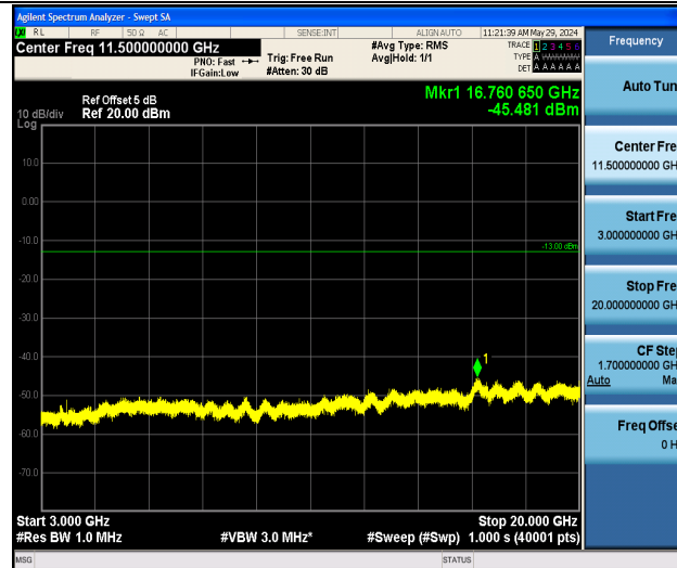
Band2_5MHz_QPSK_19175_1RB#0_3000~20000_3000~20000
