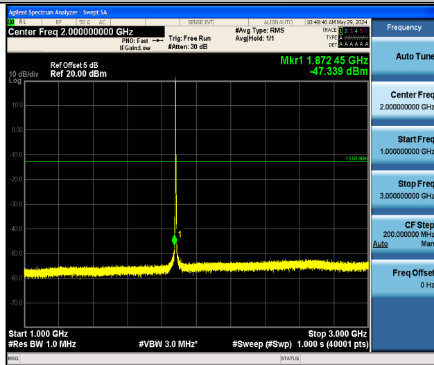
Band2_3MHz_QPSK_18900_1RB#0_1000~3000_1000~3000
