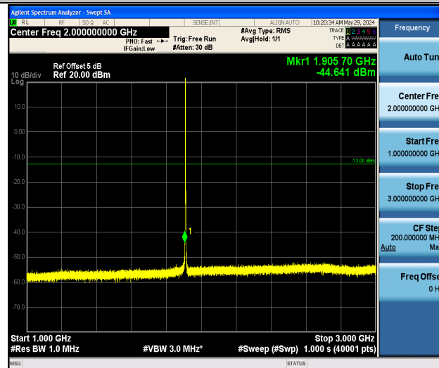
Band2_1.4MHz_16QAM_19193_1RB#0_1000~3000_1000~3000
