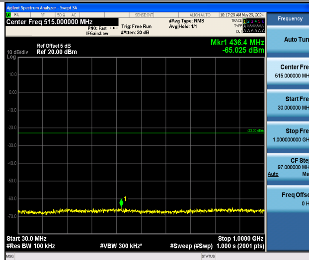
Band2_1.4MHz_QPSK_18900_1RB#0_30~1000_30~1000
