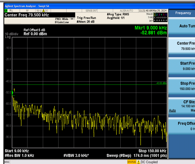
Band2_5MHz_16QAM_19175_1RB#0_0.009~0.15_0.009~0.15
