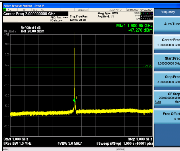
Band2_3MHz_QPSK_19185_1RB#0_1000~3000_1000~3000
