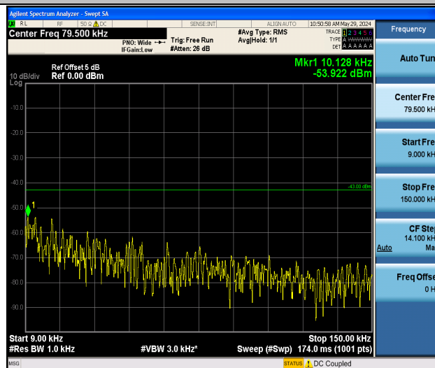
Band2_3MHz_16QAM_19185_1RB#0_0.009~0.15_0.009~0.15
