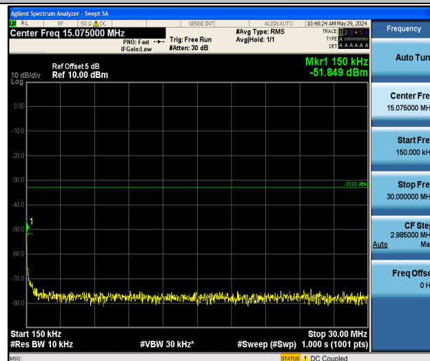
Band2_3MHz_QPSK_18900_1RB#0_0.15~30_0.15~30
