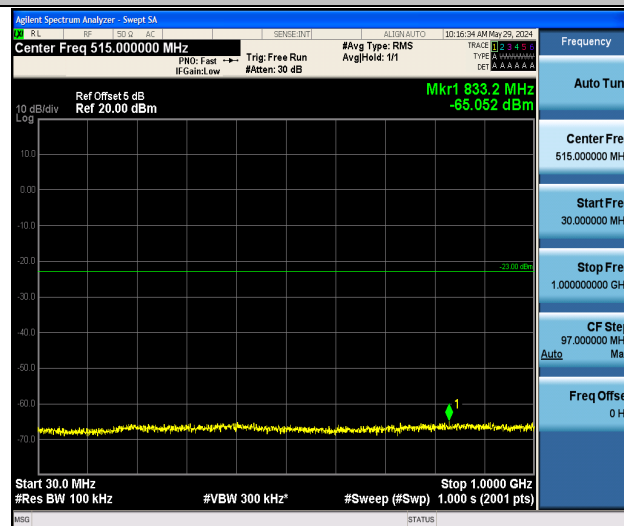
Band2_1.4MHz_16QAM_18607_1RB#0_30~1000_30~1000
