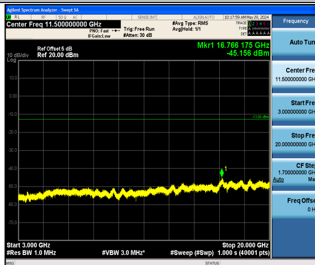
Band2_1.4MHz_QPSK_18900_1RB#0_3000~20000_3000~20000
