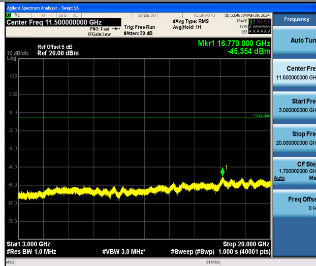
Band2_3MHz_QPSK_19185_1RB#0_3000~20000_3000~20000
