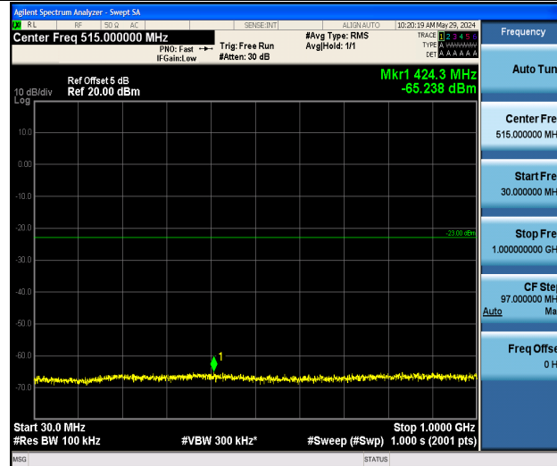
Band2_1.4MHz_16QAM_19193_1RB#0_30~1000_30~1000
