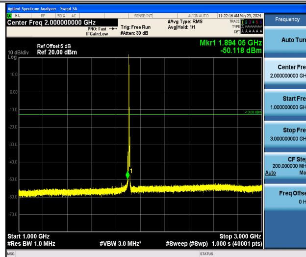
Band2_5MHz_16QAM_19175_1RB#0_1000~3000_1000~3000
