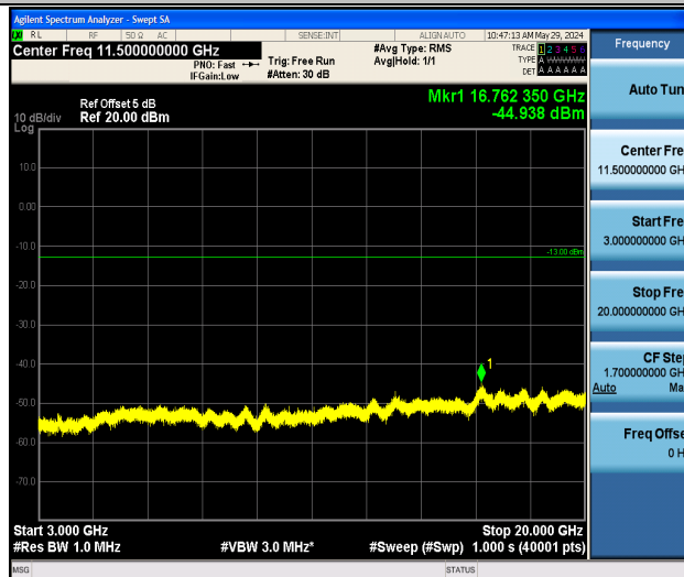
Band2_3MHz_QPSK_18615_1RB#0_3000~20000_3000~20000
