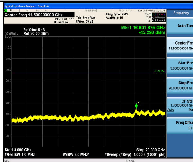
Band2_3MHz_16QAM_19185_1RB#0_3000~20000_3000~20000
