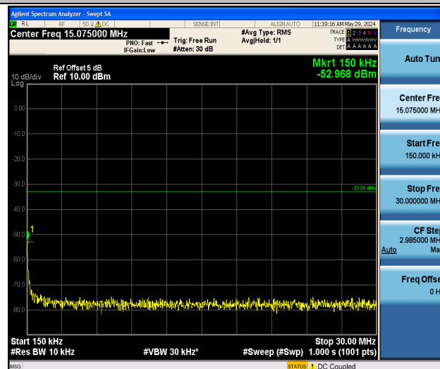
Band2_5MHz_QPSK_18900_1RB#0_0.15~30_0.15~30
