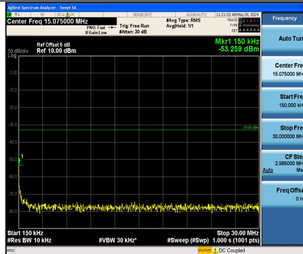
Band2_5MHz_QPSK_19175_1RB#0_0.15~30_0.15~30
