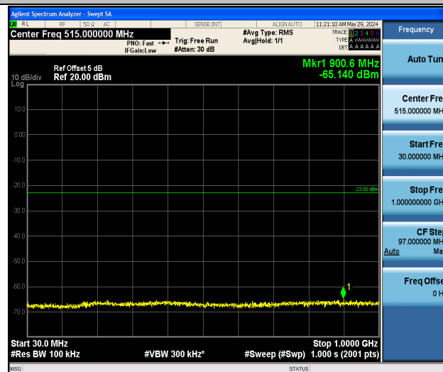
Band2_5MHz_QPSK_19175_1RB#0_30~1000_30~1000
