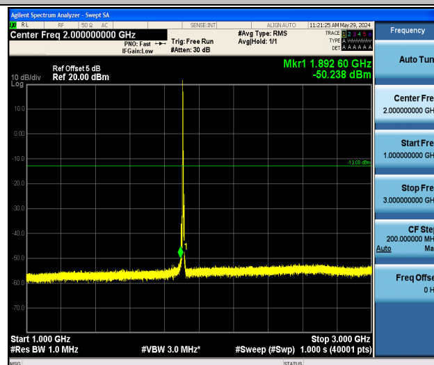
Band2_5MHz_QPSK_19175_1RB#0_1000~3000_1000~3000
