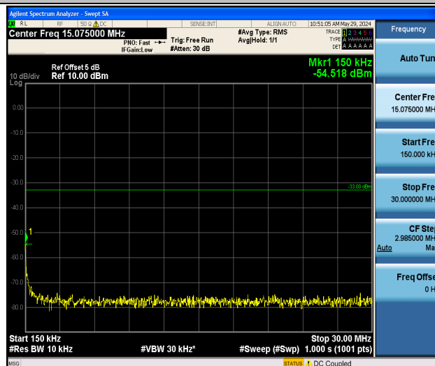
Band2_3MHz_16QAM_19185_1RB#0_0.15~30_0.15~30
