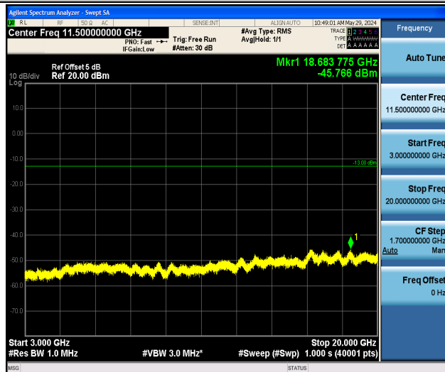
Band2_3MHz_QPSK_18900_1RB#0_3000~20000_3000~20000
