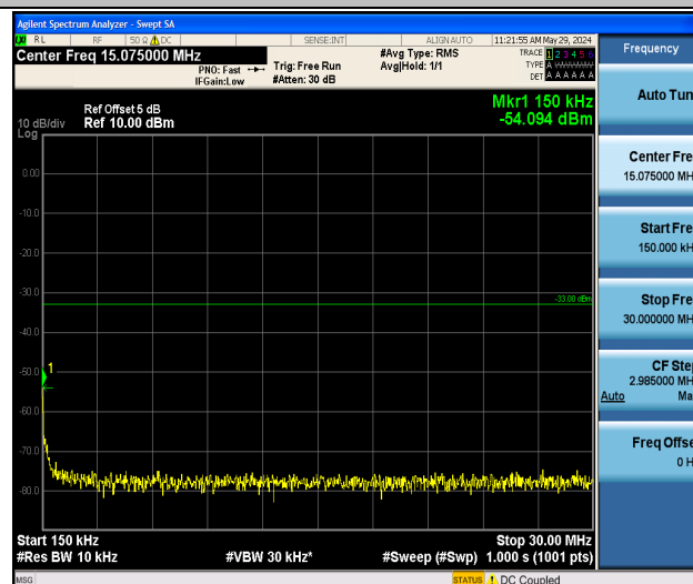
Band2_5MHz_16QAM_19175_1RB#0_0.15~30_0.15~30
