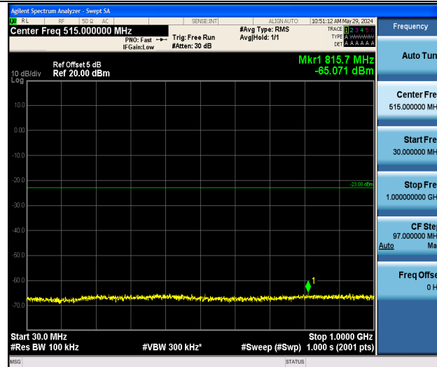
Band2_3MHz_16QAM_19185_1RB#0_30~1000_30~1000
