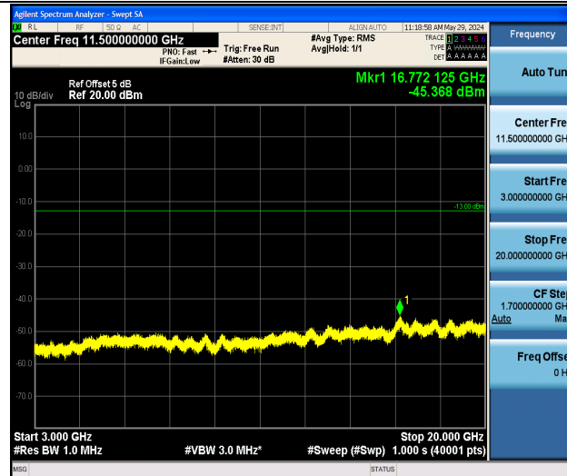
Band2_5MHz_16QAM_18625_1RB#0_3000~20000_3000~20000
