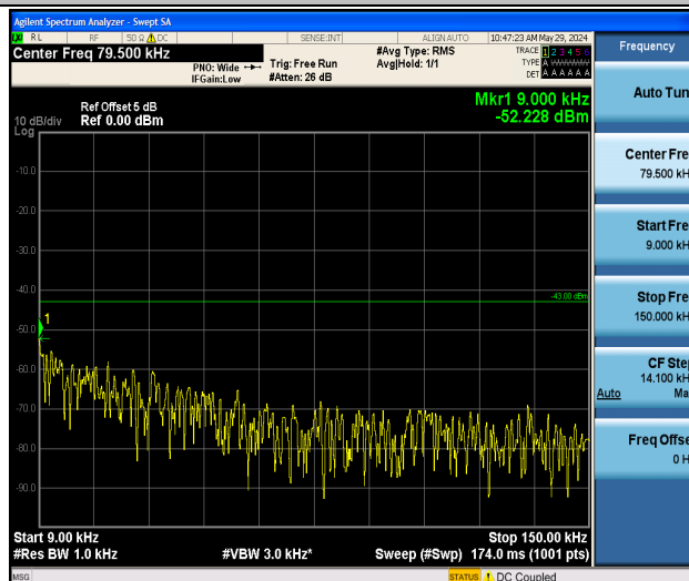
Band2_3MHz_16QAM_18615_1RB#0_0.009~0.15_0.009~0.15
