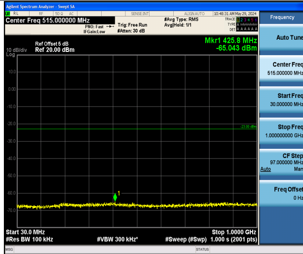
Band2_3MHz_QPSK_18900_1RB#0_30~1000_30~1000
