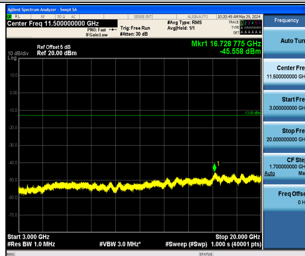
Band2_1.4MHz_16QAM_19193_1RB#0_3000~20000_3000~20000
