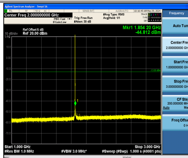
Band2_1.4MHz_16QAM_18607_1RB#0_1000~3000_1000~3000
