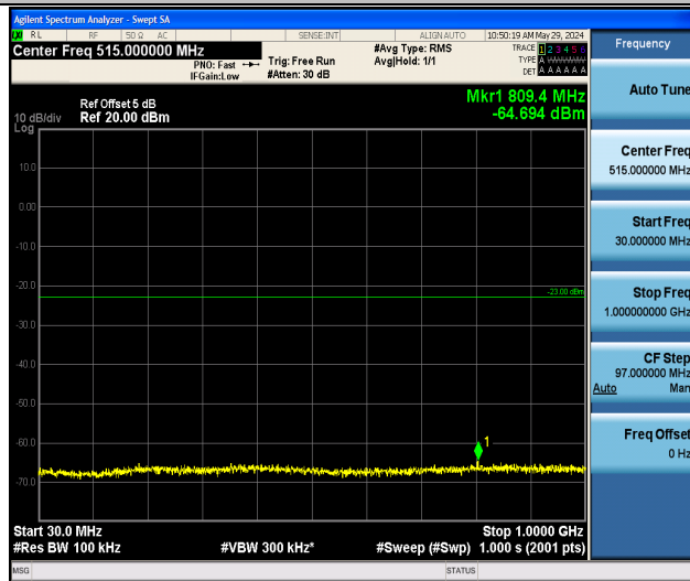
Band2_3MHz_QPSK_19185_1RB#0_30~1000_30~1000
