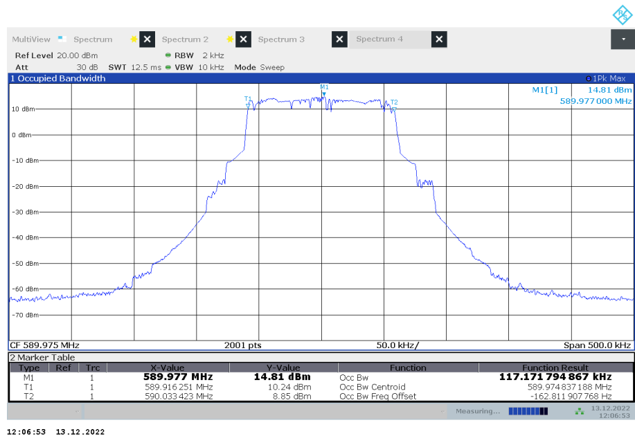
Plot 3: 589.975 MHz, max hold with frequency variation from 50 Hz to 15 kHz
