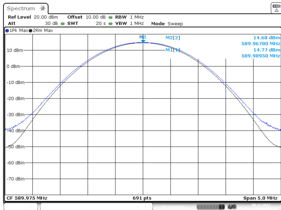
Plot 3: 589.975 MHz (modulated carrier)
