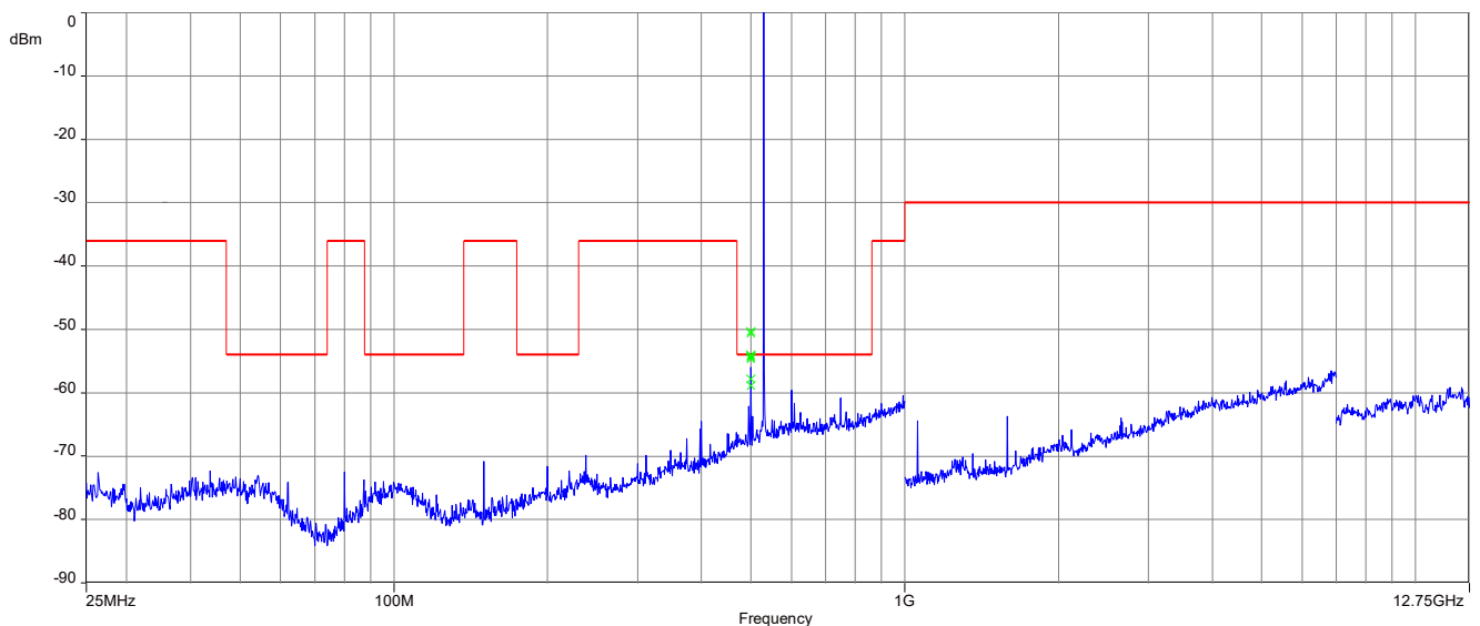
Plot 1: 530.000 MHz, spurious emissions, 25 MHz – 12.75 GHz
