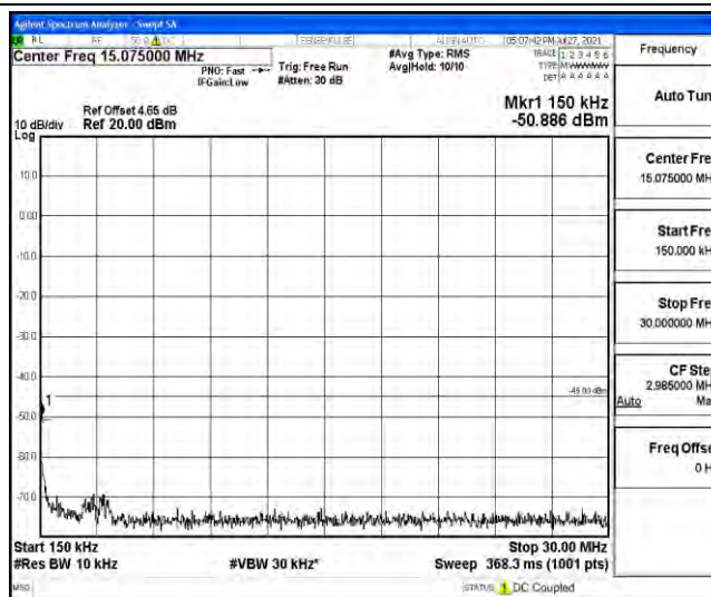
Band38-20MHz-QPSK-38150-1RB#0-Range3:30~1000MHz
