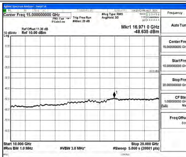
Band38-15MHz-QPSK-37825-1RB#0-Range6:20000~26500MHz
