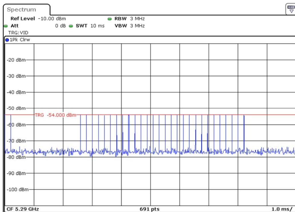
Radar Type 2 Calibration Plot (5290MHz)
