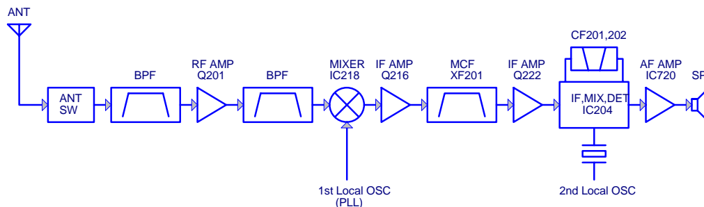
Fig.3 Receiver Section Configuration
