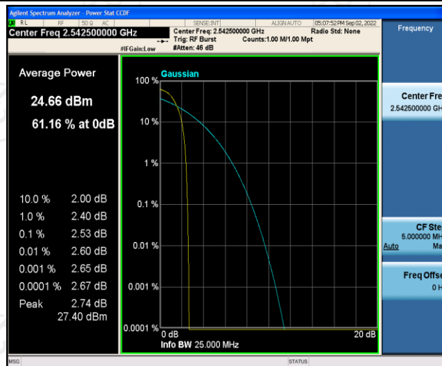
Band41-15MHz-QPSK-40115-75RB#0
