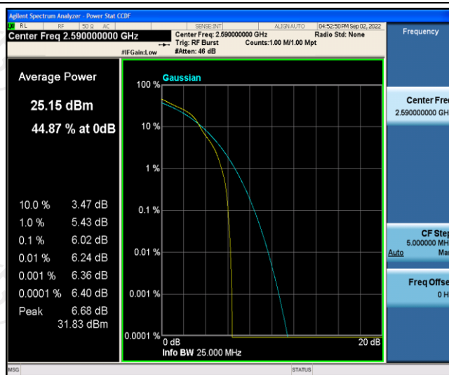
Band41-10MHz-16QAM-40590-50RB#0
