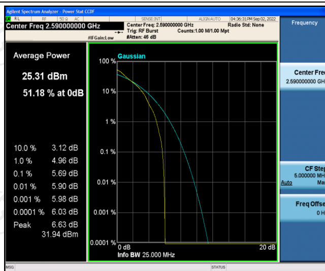
Band41-5MHz-QPSK-40590-25RB#0
