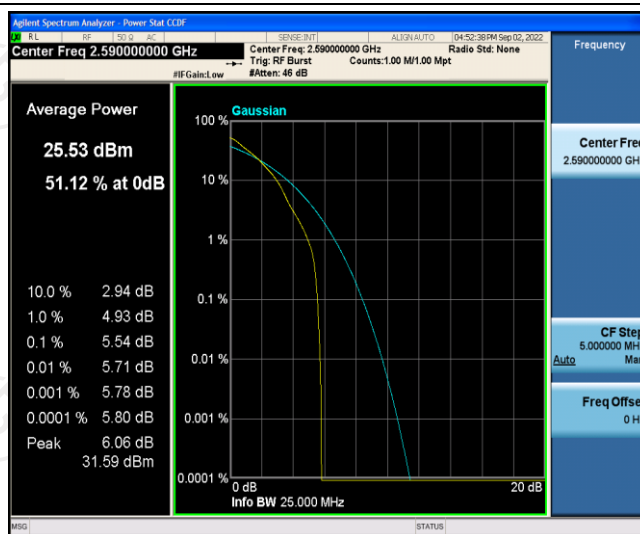
Band41-10MHz-QPSK-40590-50RB#0
