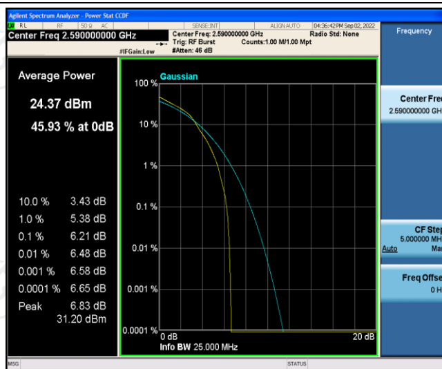
Band41-5MHz-16QAM-40590-25RB#0
