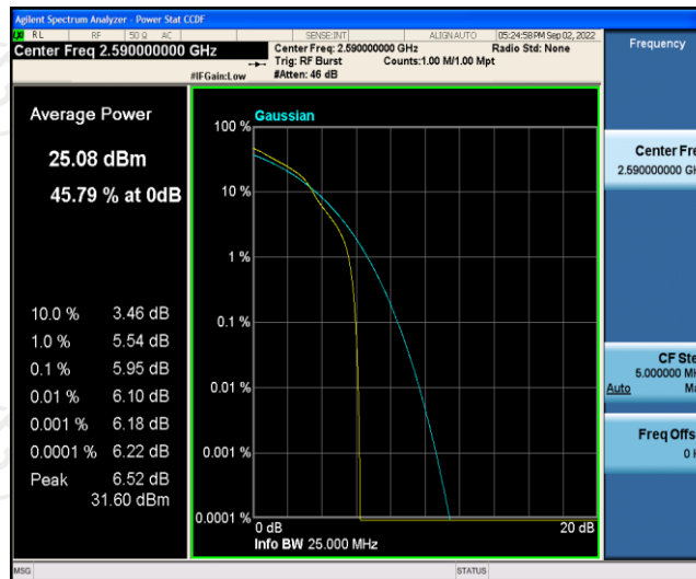
Band41-20MHz-16QAM-40590-100RB#0
