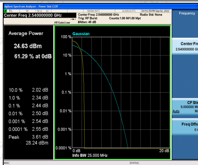
Band41-10MHz-QPSK-40090-50RB#0
