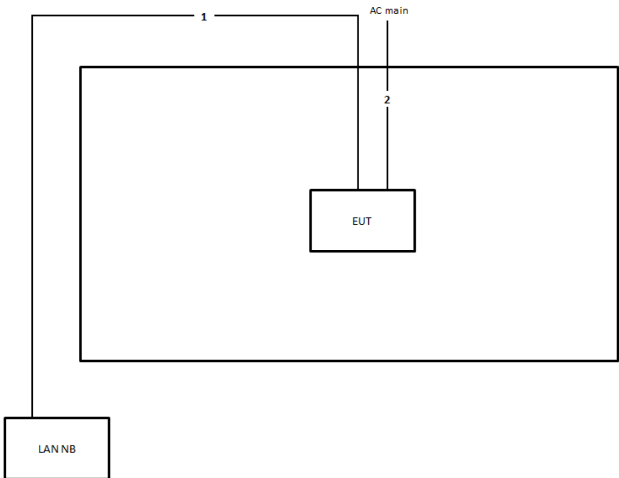
Test Setup Diagram - Radiated Test > 1GHz / For non-beamforming mode
