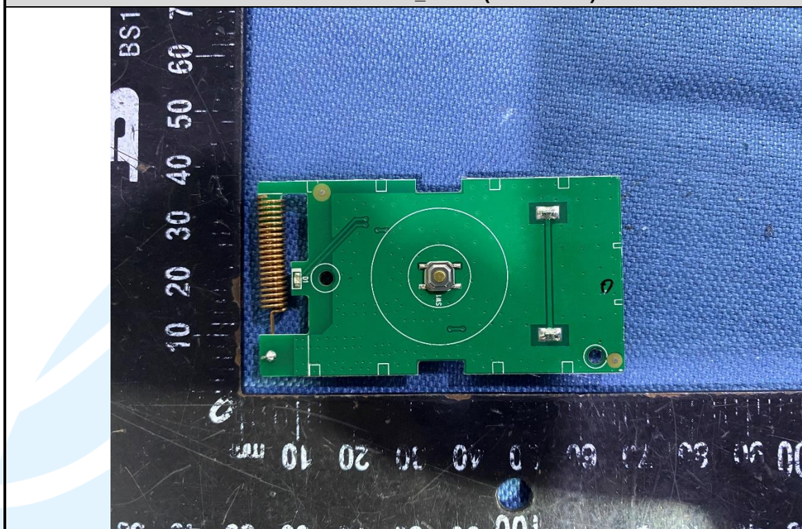
EUT Photo_CB-21 (Transmitter)
