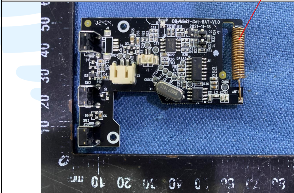
EUT Photo_WA-11 (Receiver)
