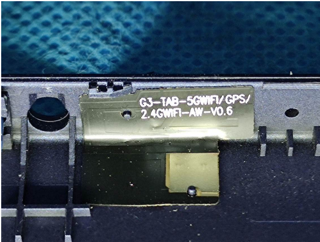
WLAN/Bluetooth Antenna
