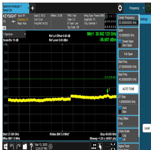
NTNV-n77(3700-3980)-PC2-30-100-H-DFT-BPSK- Edge_1RB_Left-27000-40000-PASS
