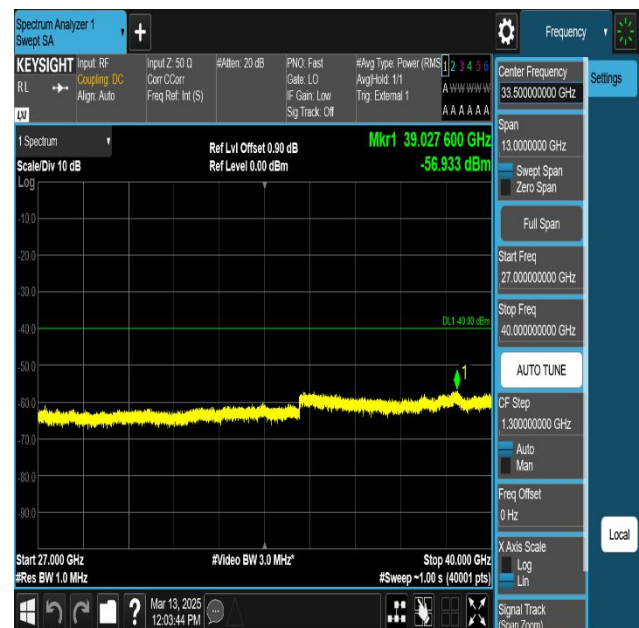
NTNV-n77(3700-3980)-PC2-30-100-M-CP-QPSK- Edge_1RB_Left-27000-40000-PASS
