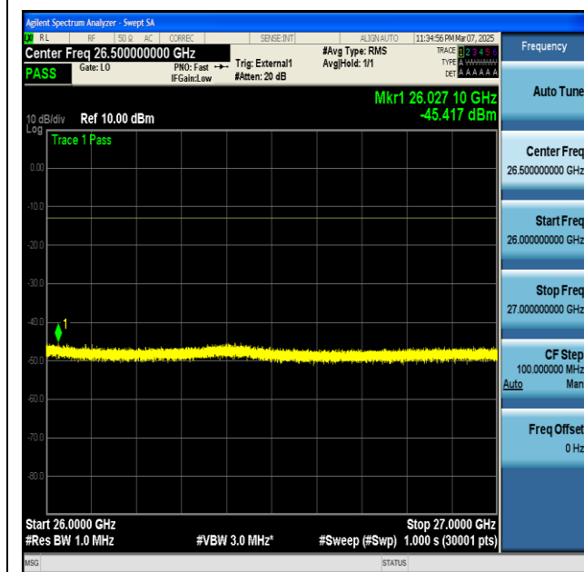
NTNV-n77(3700-3980)-PC2-30-100-L-DFT-BPSK- Edge_1RB_Left-26000-27000-PASS
