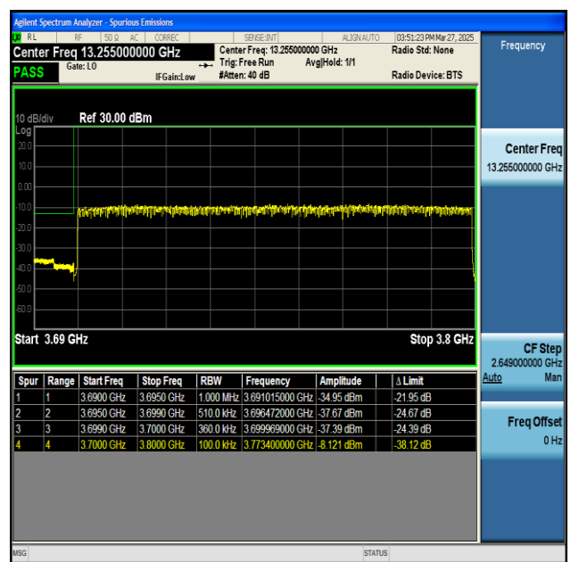
NTNV-n77(3700-3980)-PC2-30-100-L-CP-QPSK- Outer_Full-PASS
