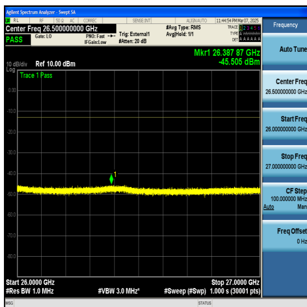
NTNV-n77(3700-3980)-PC2-30-100-H-DFT-BPSK- Edge_1RB_Left-26000-27000-PASS
