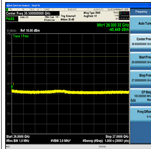
NTNV-n77(3700-3980)-PC2-30-100-H-CP-QPSK- Edge_1RB_Left-26000-27000-PASS
