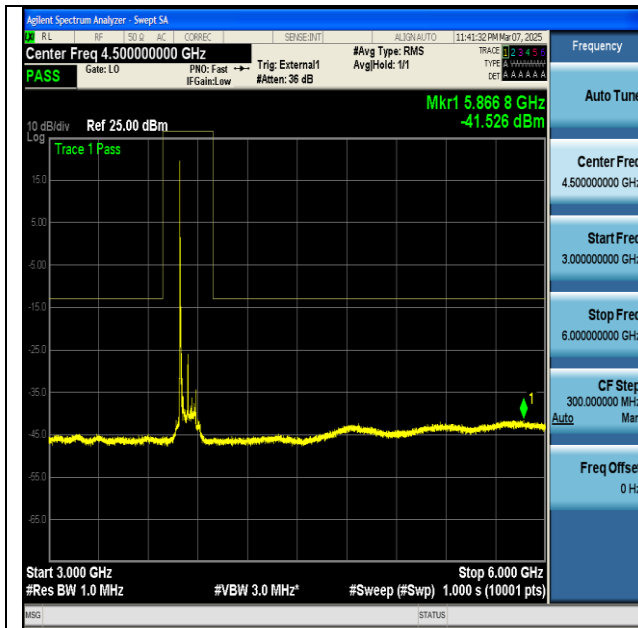
NTNV-n77(3700-3980)-PC2-30-100-M-CP-QPSK- Edge_1RB_Left-3000-6000-PASS
