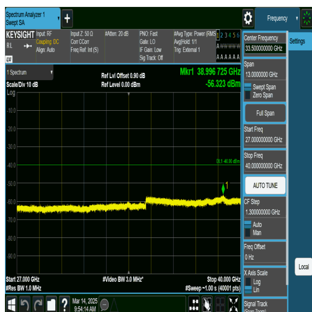
NTNV-n77(3700-3980)-PC2-30-100-M-DFT-BPSK- Edge_1RB_Left-27000-40000-PASS
