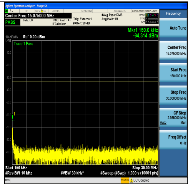
NTNV-n77(3700-3980)-PC2-30-100-M-CP-QPSK- Edge_1RB_Left-0.15-30-PASS
