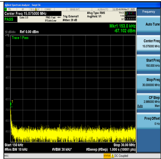
NTNV-n77(3700-3980)-PC2-30-100-L-CP-QPSK- Edge_1RB_Left-0.15-30-PASS
