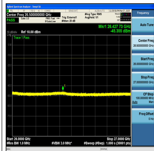
NTNV-n77(3700-3980)-PC2-30-100-M-DFT-BPSK- Edge_1RB_Left-26000-27000-PASS
