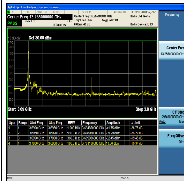
NTNV-n77(3700-3980)-PC2-30-100-L-CP-QPSK- Edge_1RB_Left-PASS
