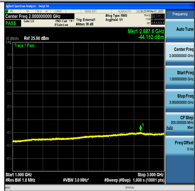
NTNV-n77(3700-3980)-PC2-30-100-L-CP-QPSK- Edge_1RB_Left-1000-3000-PASS
