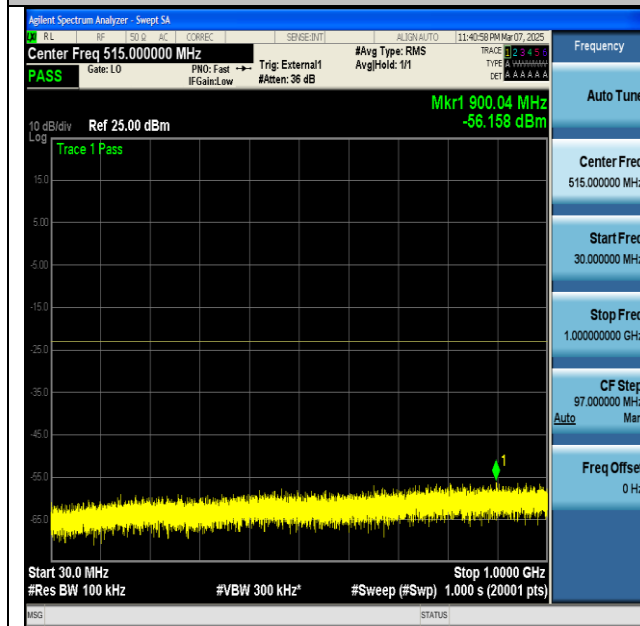
NTNV-n77(3700-3980)-PC2-30-100-M-CP-QPSK- Edge_1RB_Left-30-1000-PASS
