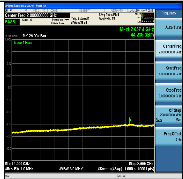
NTNV-n77(3700-3980)-PC2-30-100-M-CP-QPSK- Edge_1RB_Left-1000-3000-PASS
