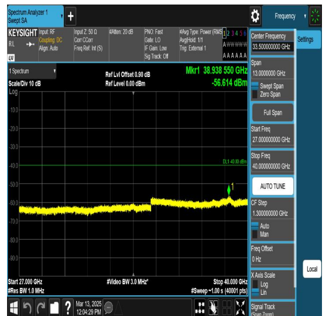
NTNV-n77(3700-3980)-PC2-30-100-H-CP-QPSK- Edge_1RB_Left-27000-40000-PASS
