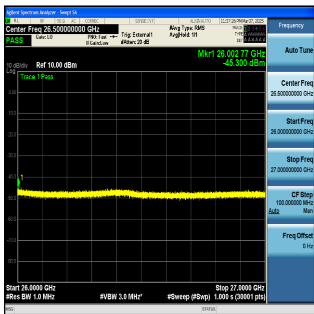
NTNV-n77(3700-3980)-PC2-30-100-L-CP-QPSK- Edge_1RB_Left-26000-27000-PASS
