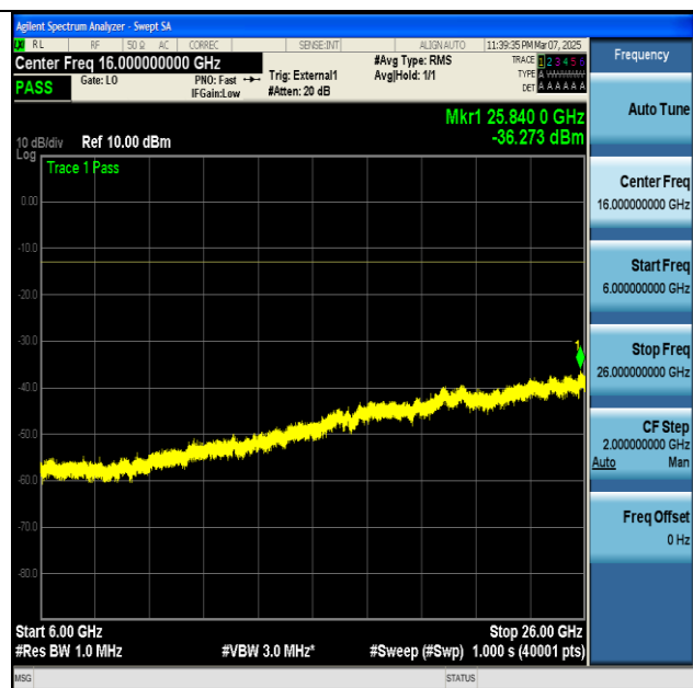
NTNV-n77(3700-3980)-PC2-30-100-M-DFT-BPSK- Edge_1RB_Left-6000-26000-PASS
