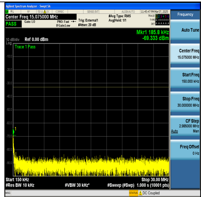
NTNV-n77(3700-3980)-PC2-30-100-H-CP-QPSK- Edge_1RB_Left-0.15-30-PASS
