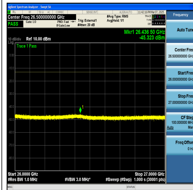
NTNV-n77(3700-3980)-PC2-30-100-M-CP-QPSK- Edge_1RB_Left-26000-27000-PASS
