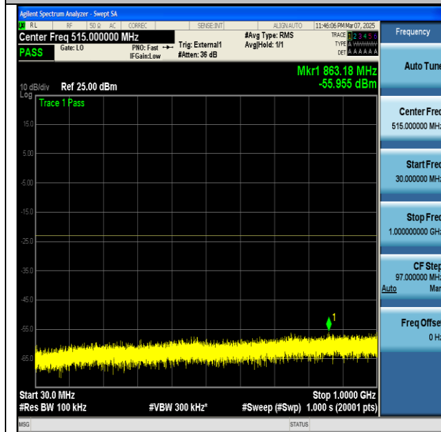
NTNV-n77(3700-3980)-PC2-30-100-H-CP-QPSK- Edge_1RB_Left-30-1000-PASS
