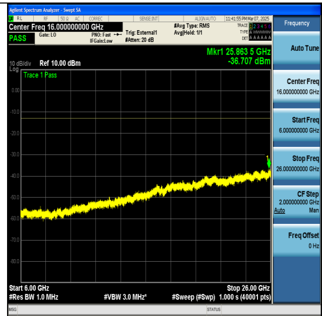
NTNV-n77(3700-3980)-PC2-30-100-M-CP-QPSK- Edge_1RB_Left-6000-26000-PASS
