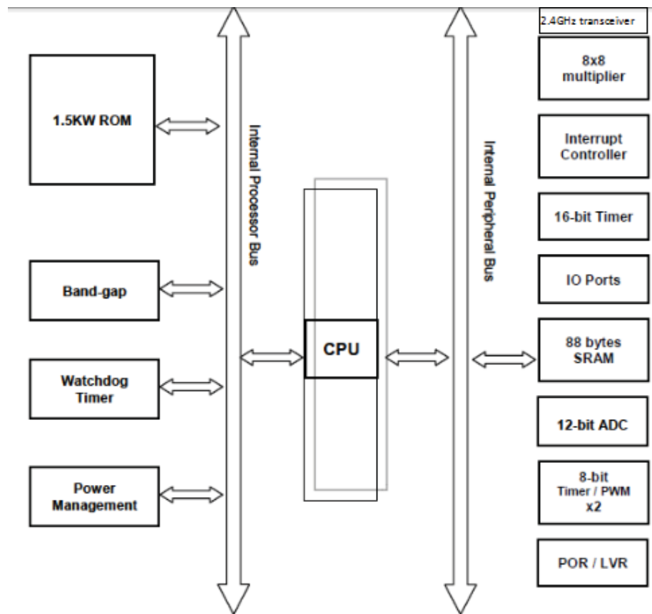
Chart1 FW1210 SOC block diagram
