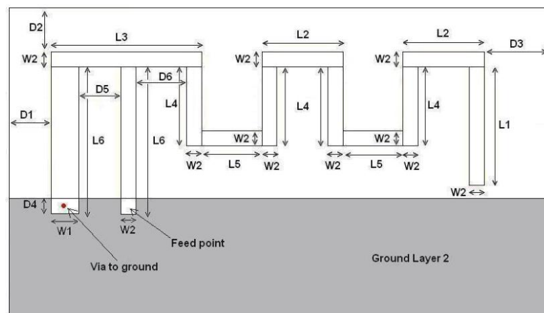
Figure 1: Antenna Dimensions
