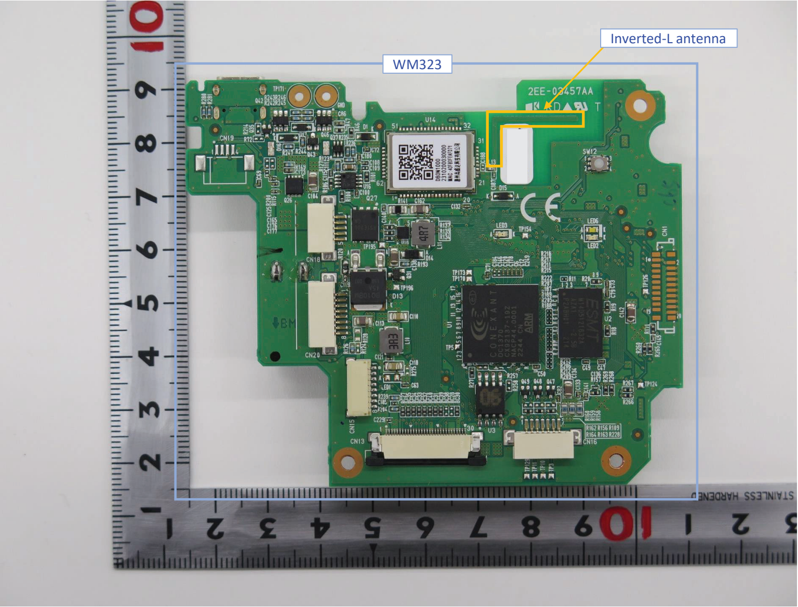
■Antenna position of WM323
