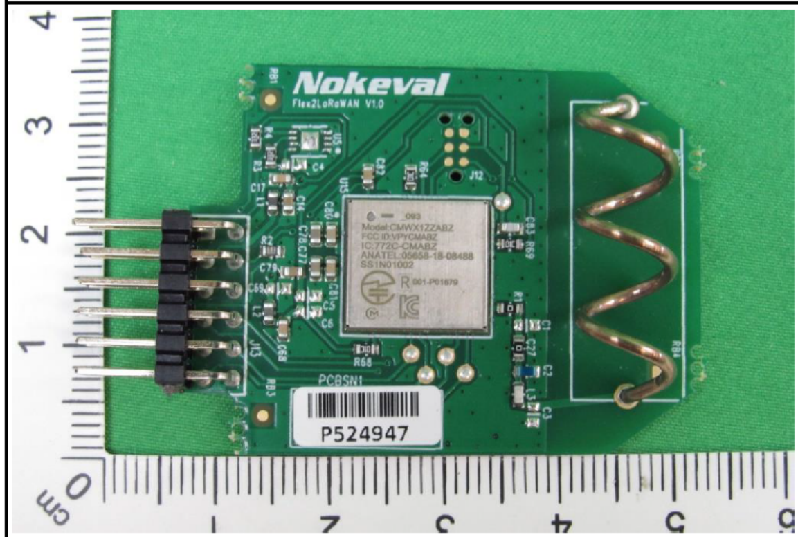
Model Flex2-Radio-LWNA PCB front view
