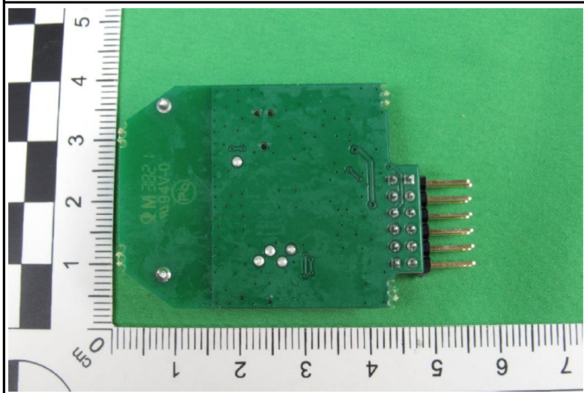
Model Flex2-Radio-LWNA PCB back view
