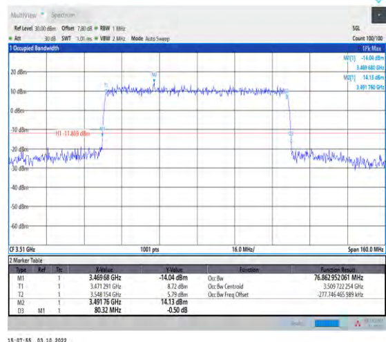
1-N78-3450-3550--30-80-H-4-DFT-64QAM-Outer_Full -216@0-Ant1-76.863-80.320-≤80-PASS
