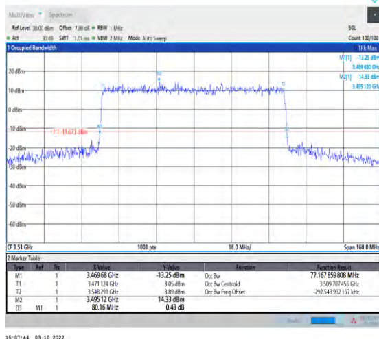
1-N78-3450-3550--30-80-H-3-DFT-16QAM-Outer_Full -216@0-Ant1-77.168-80.160-≤80-PASS
