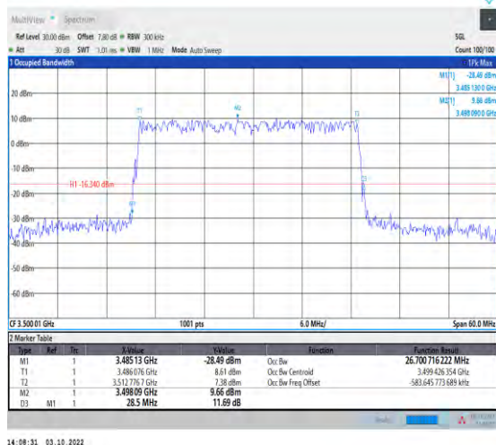
1-N78-3450-3550--30-30-M-5-DFT-256QAM-Outer_Full-75@0-Ant1-26.701-28.500-<30-PASS
