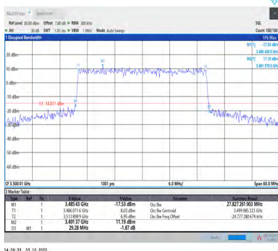
1-N78-3450-3550--30-30-M-8-CP-64QAM-Outer_Full -78@0-Ant1-27.827-29.280-<30-PASS
