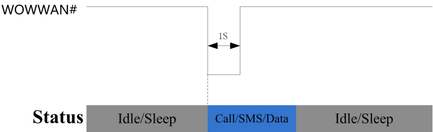
Figure 3-15 WOWWAN# Timing
