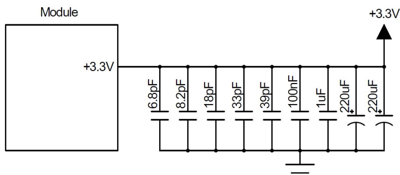
Figure 3-2 Power Supply Design
