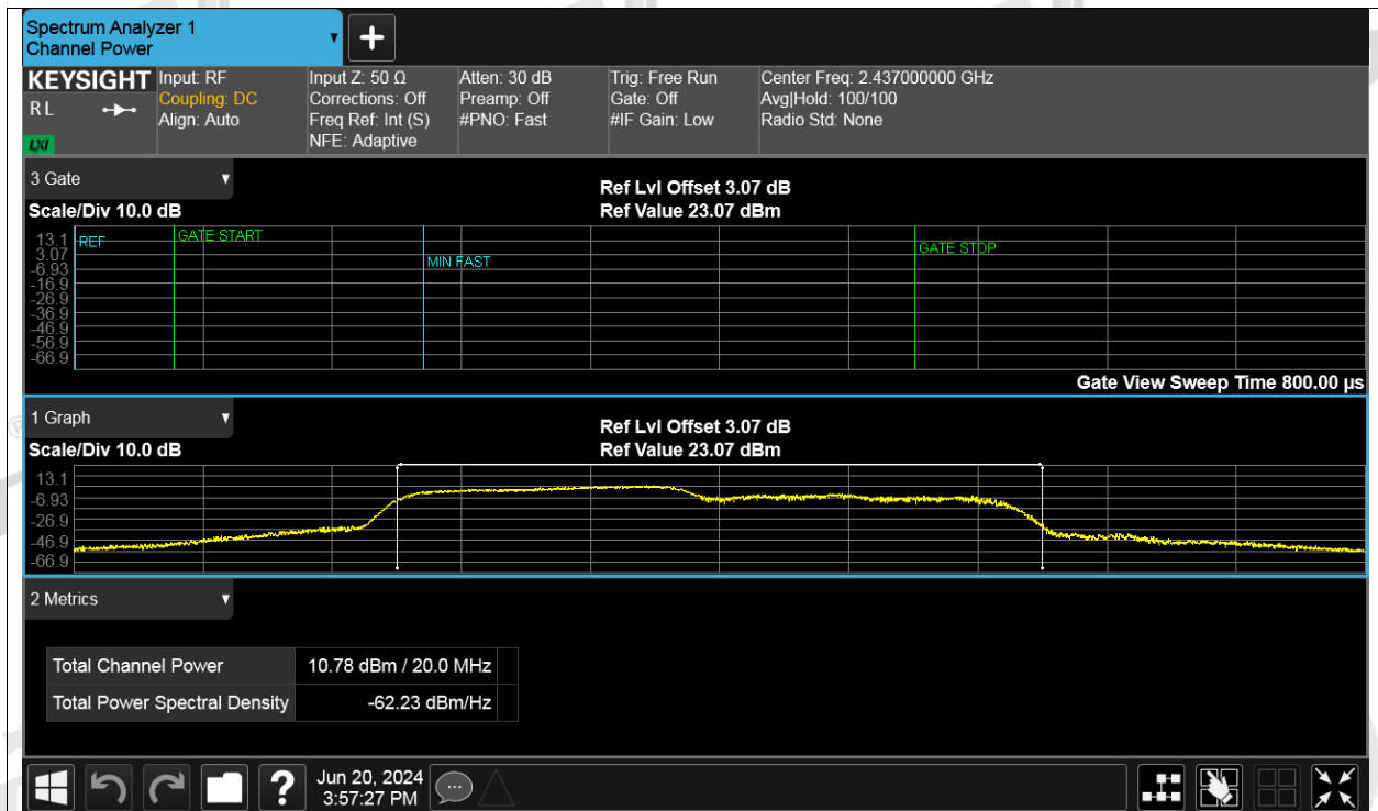
Power NVNT ax20 106RU Index 53 2437MHz Ant2
