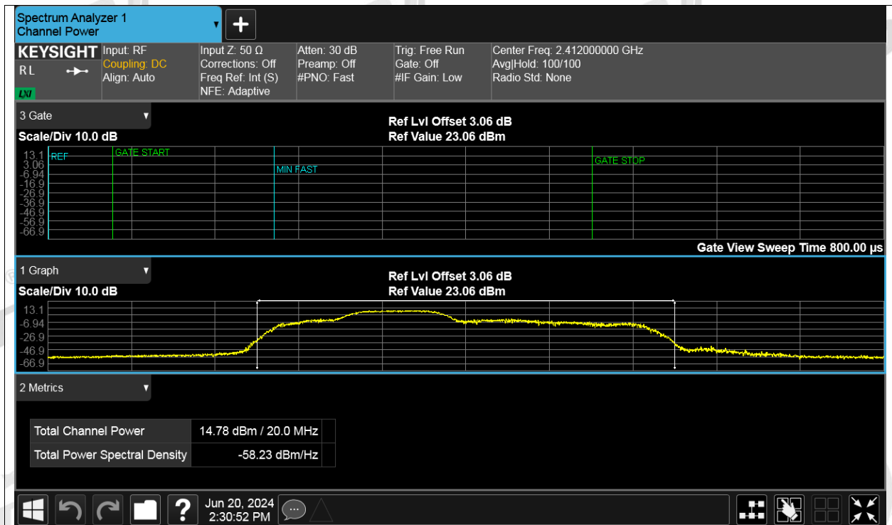
Power NVNT ax20 52RU Index 37 2412MHz Ant2
