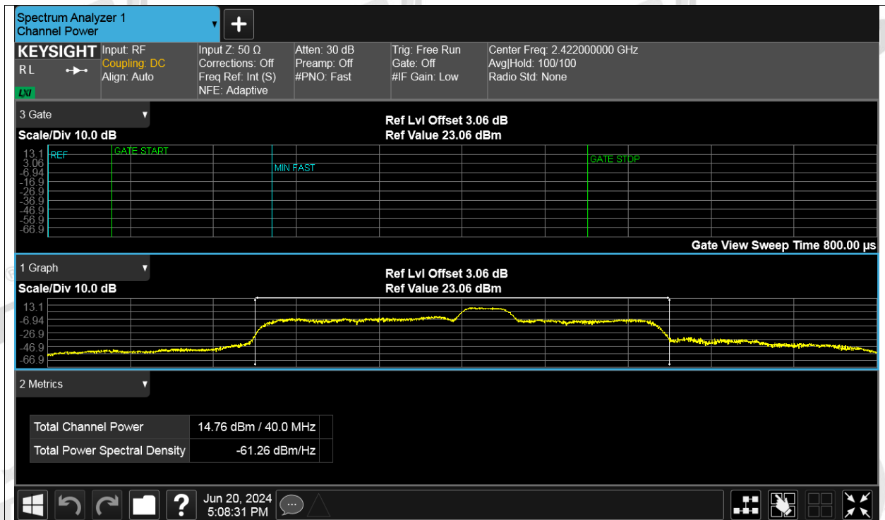
Power NVNT ax40 52RU Index 41 2422MHz Ant2
