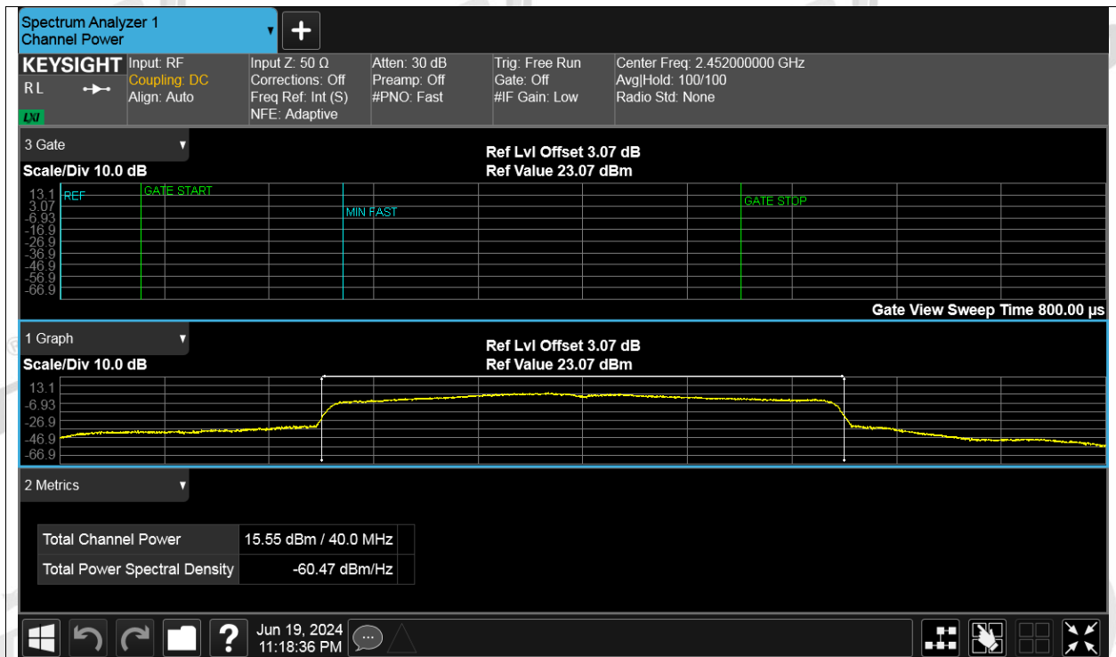
Power NVNT be40 2452MHz Ant2
