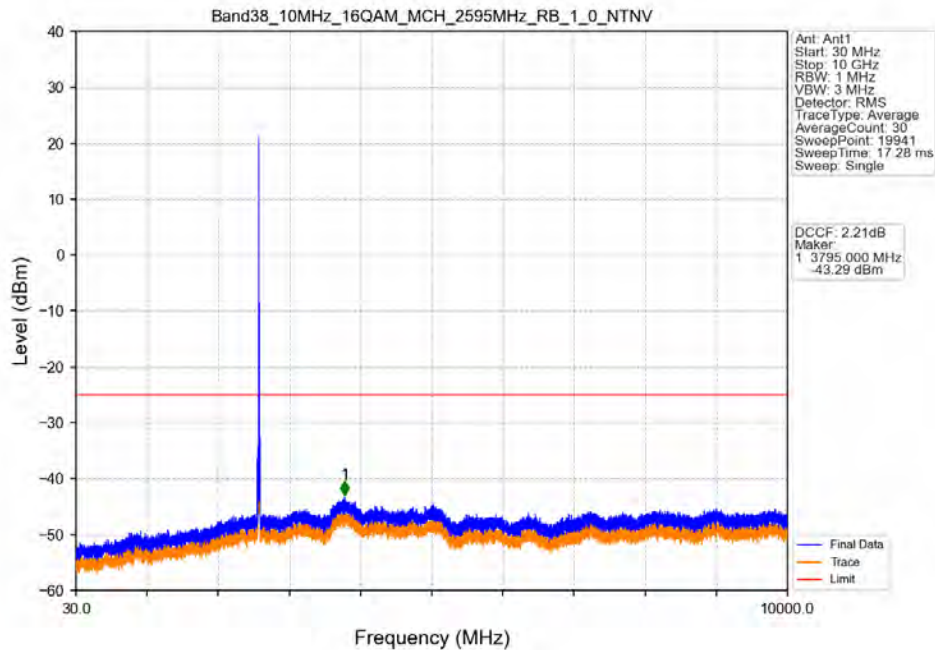
Band38_10MHz_16QAM_MCH_2595MHz_RB_1_0_NTNV
