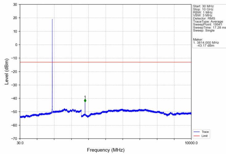
Band2_RMC_HCH_1907.6MHz_12.2kbps_RMC_NTNV
