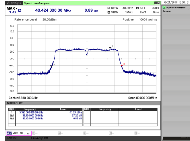
[ 802.11ac (VHT40)/ 5310 MHz ]
