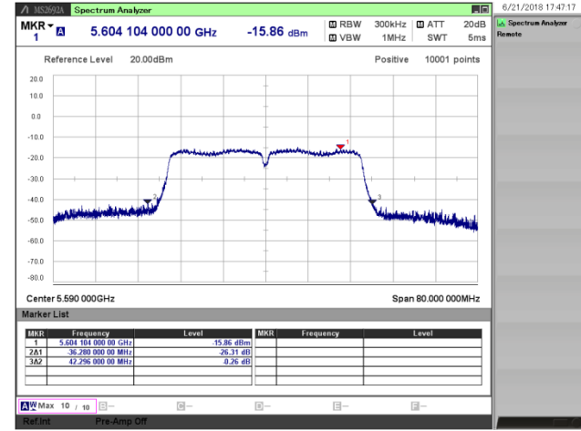
[ 802.11ac (VHT40)/ 5590 MHz ]
