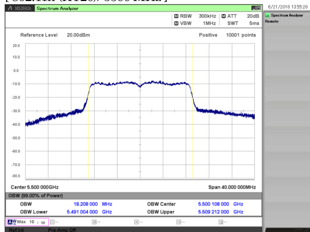
[ 802.11n (HT20)/ 5500 MHz ]
