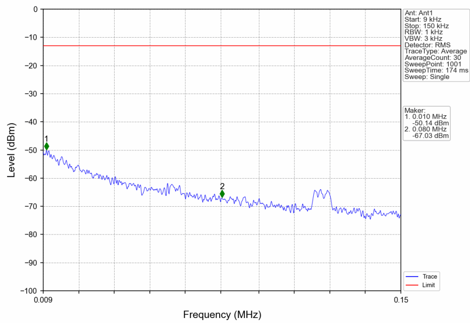
Band71_10MHz_16QAM_MCH_680.5MHz_RB_1_0_NTNV
