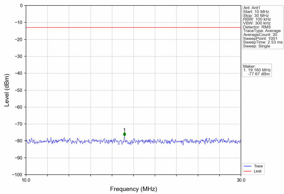
Band71_15MHz_16QAM_MCH_680.5MHz_RB_1_0_NTNV
