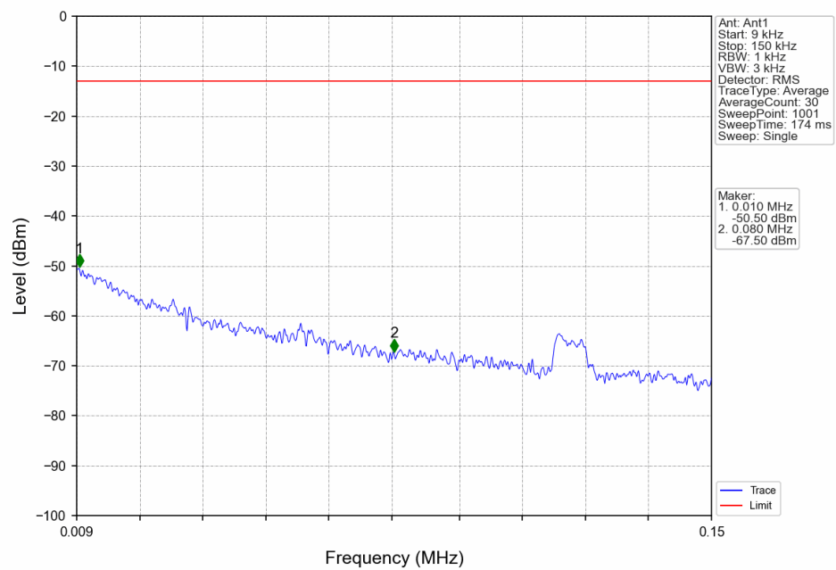
Band71_15MHz_16QAM_MCH_680.5MHz_RB_1_0_NTNV
