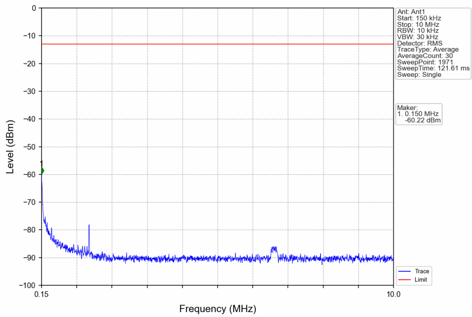
Band71_15MHz_16QAM_LCH_670.5MHz_RB_1_0_NTNV
