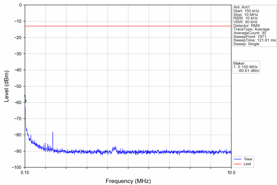
Band71_10MHz_16QAM_MCH_680.5MHz_RB_1_0_NTNV
