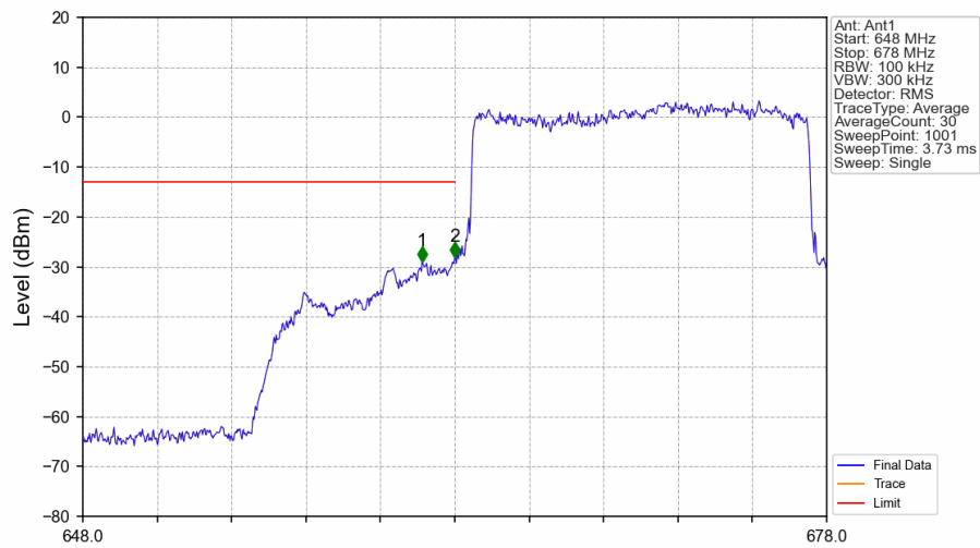
Band71_15MHz_QPSK_LCH_670.5MHz_RB_75_0_NTNV
