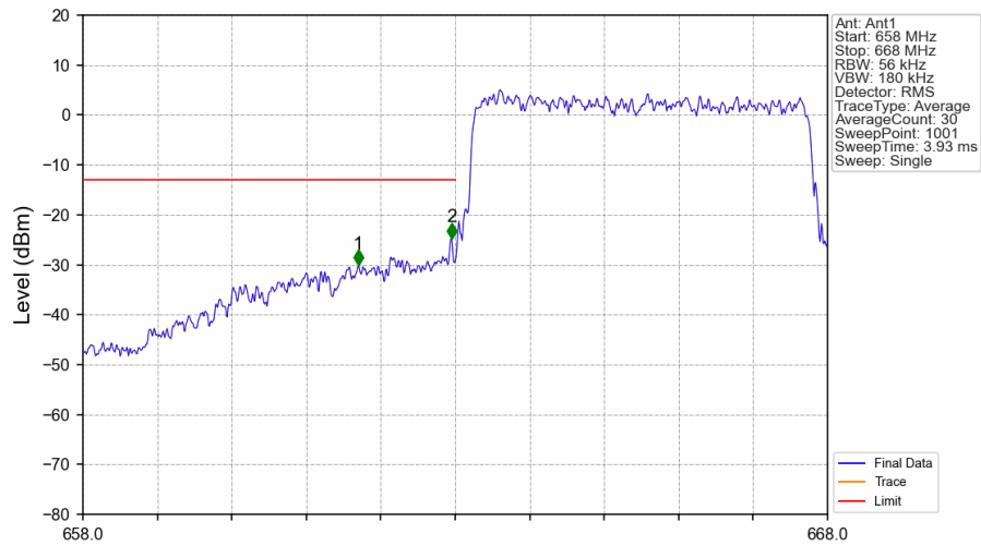
Band71_5MHz_16QAM_LCH_665.5MHz_RB_25_0_NTNV
