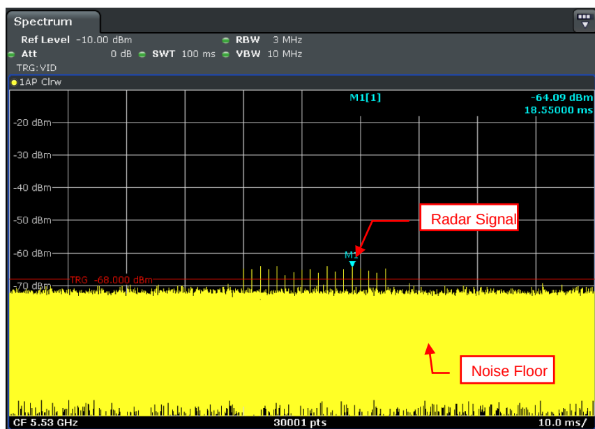
Radar Signal 0
