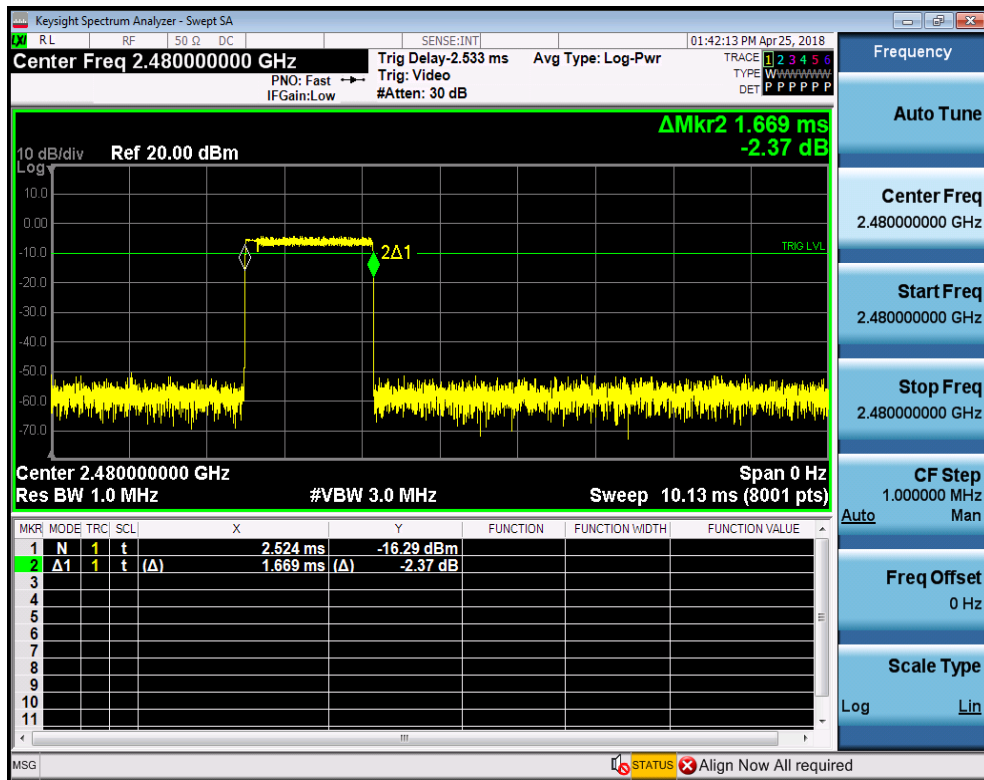
Dwell Time_3DH3_2480
