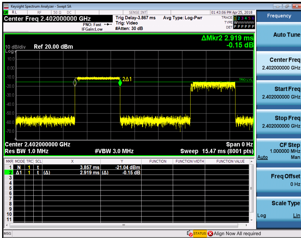
Dwell Time_3DH5_2402
