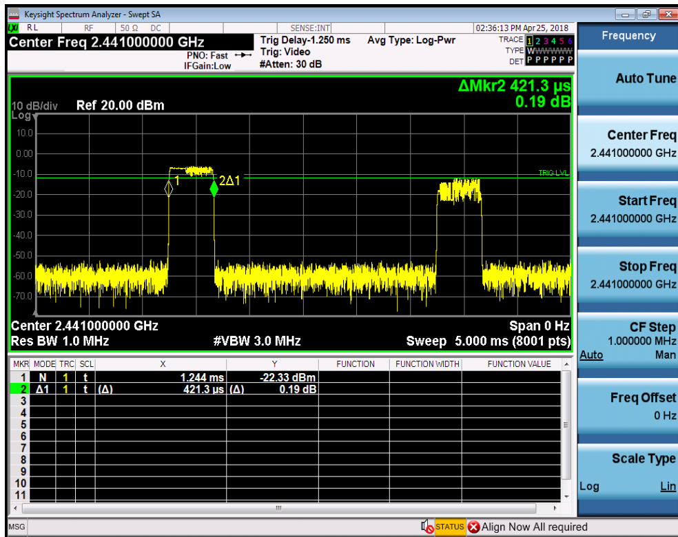
Dwell Time_2DH1_2441
