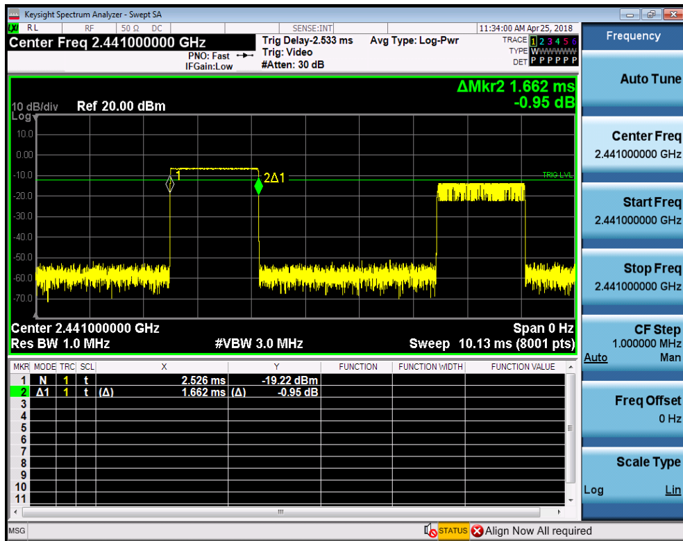
Dwell Time_DH3_2441
