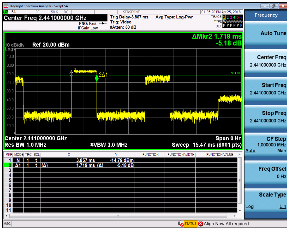
Dwell Time_2DH5_2441
