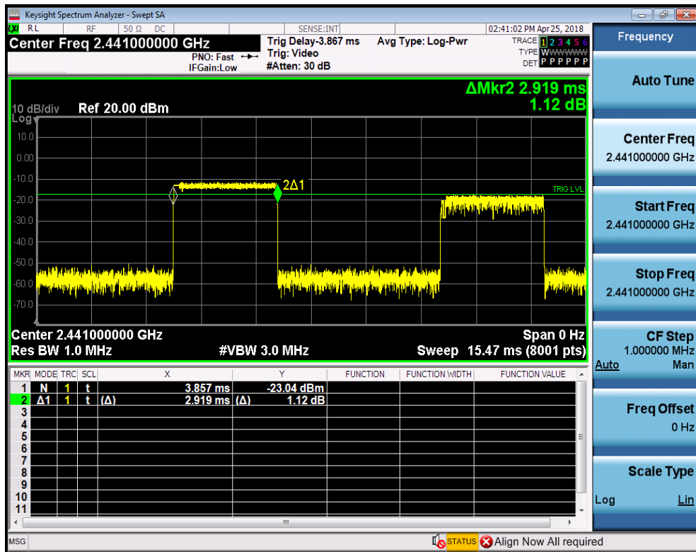
Dwell Time_3DH5_2441
