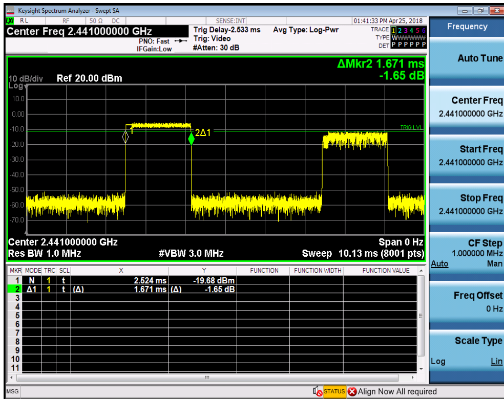
Dwell Time_3DH3_2441
