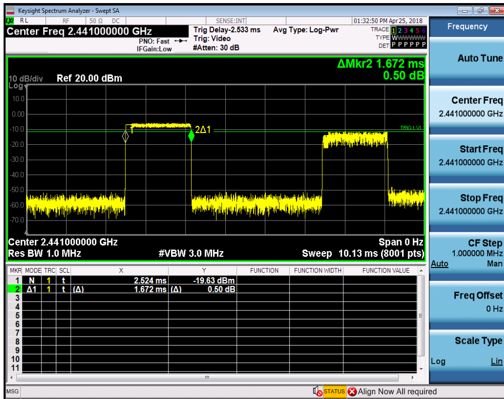
Dwell Time_2DH3_2441
