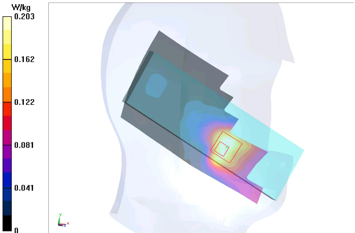
Fig.3 1900 MHz CH810
