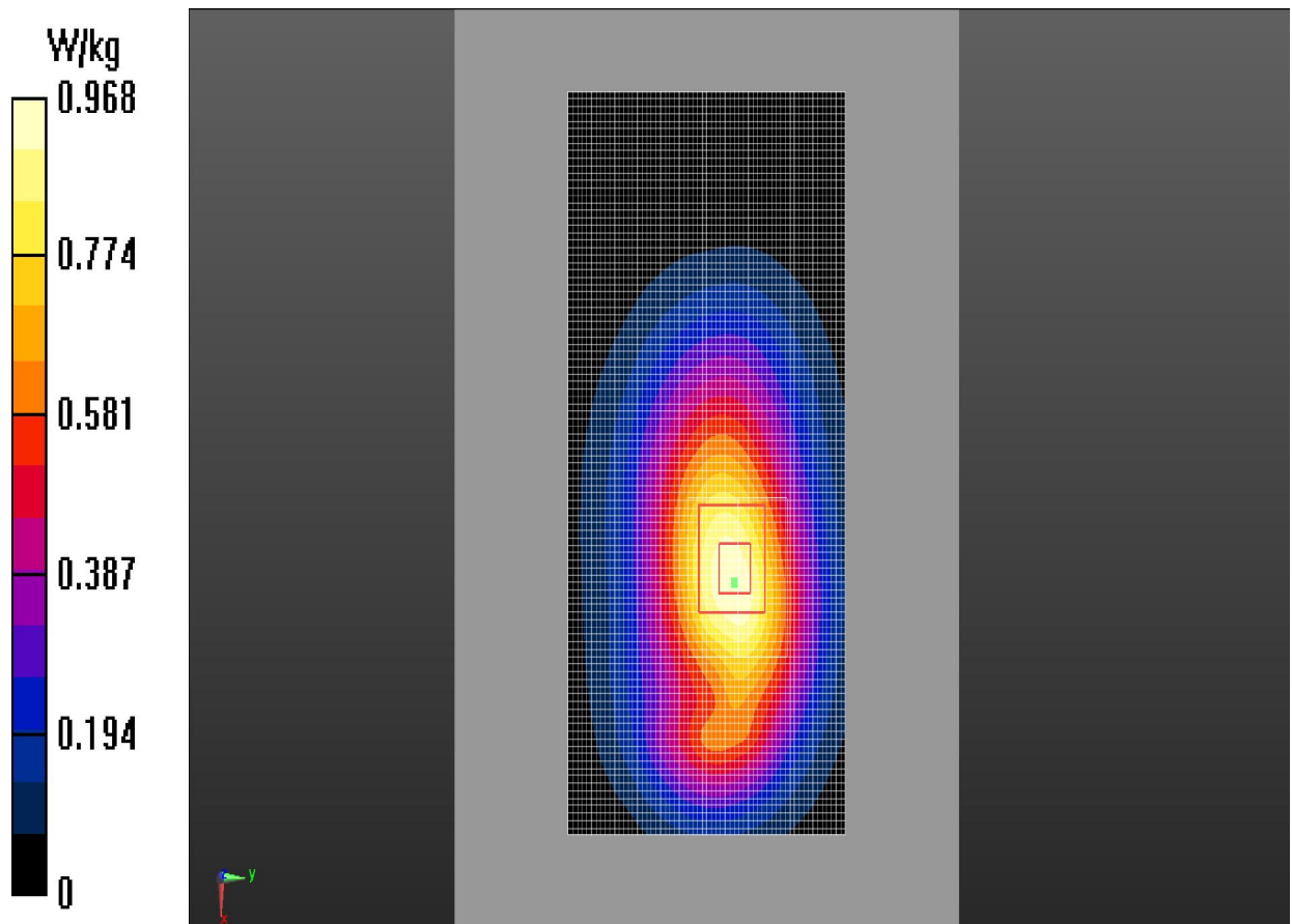
Fig.2 850 MHz CH190
