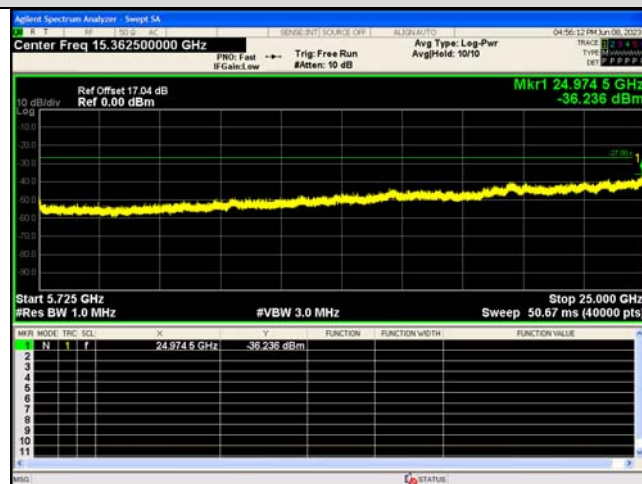
Spurious Emission:5725~25000.0 MHz IEEE 802.11n_Channel 120_20MHz_Antenna 0
