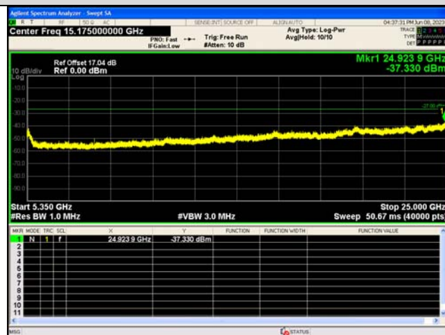
Spurious Emission:5350~25000.0 MHz IEEE 802.11n_Channel 64_20MHz_Antenna 0
