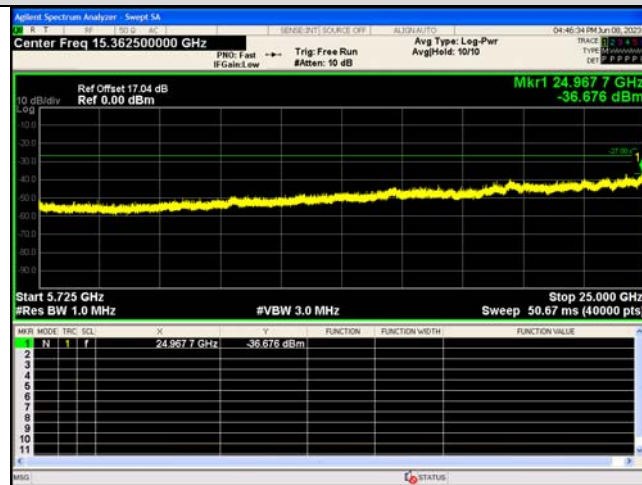
Spurious Emission:5725~25000.0 MHz IEEE 802.11a_Channel 100_20MHz_Antenna 0
