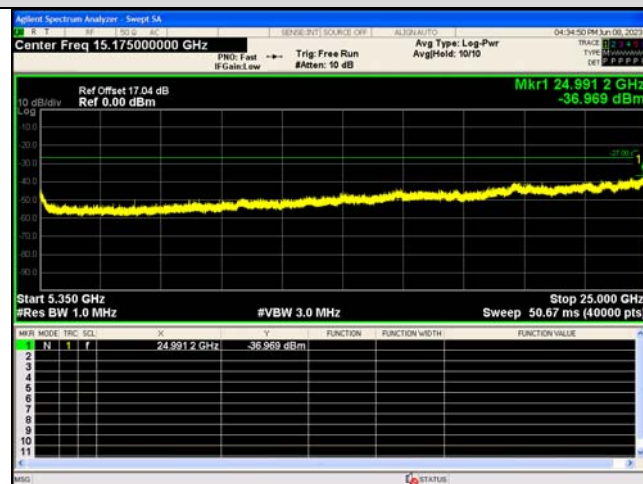
Out Of Band Emission IEEE 802.11n_Channel 56_20MHz_Antenna 0
