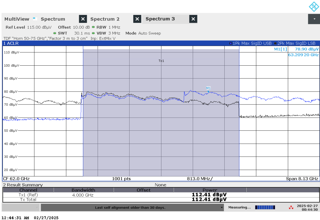
Figure 7.4-1: equivalent isotropically radiated power (EIRP) view
