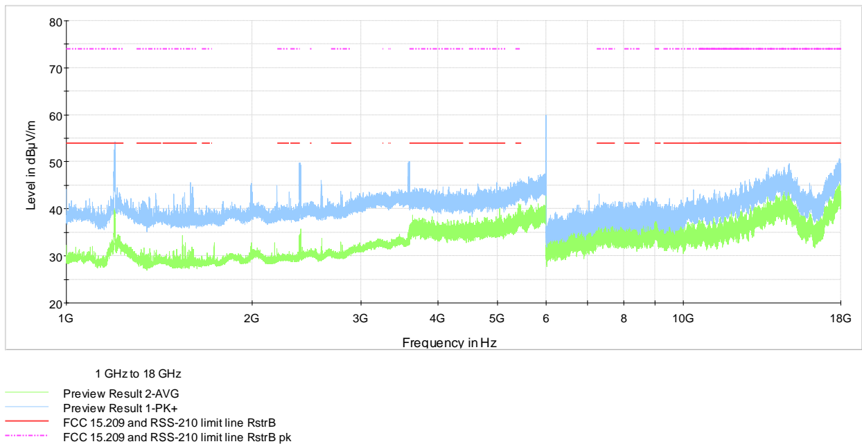
Figure 7.5-2: Radiated spurious emissions above 1-18 GHz
