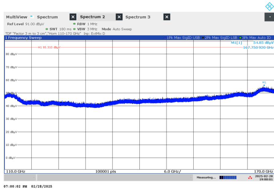
Figure 7.5-7: Radiated spurious emissions 110-170 GHz
