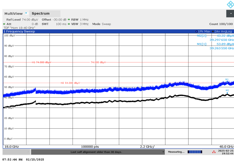
Figure 7.5-3: Radiated spurious emissions 18-40 GHz
