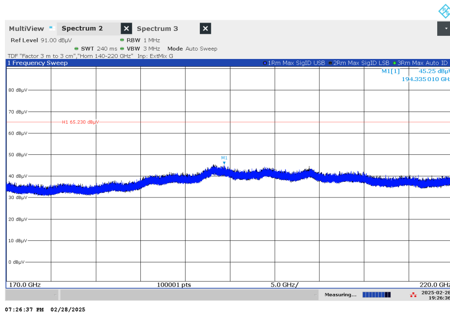
Figure 7.5-8: Radiated spurious emissions 170-220 GHz
