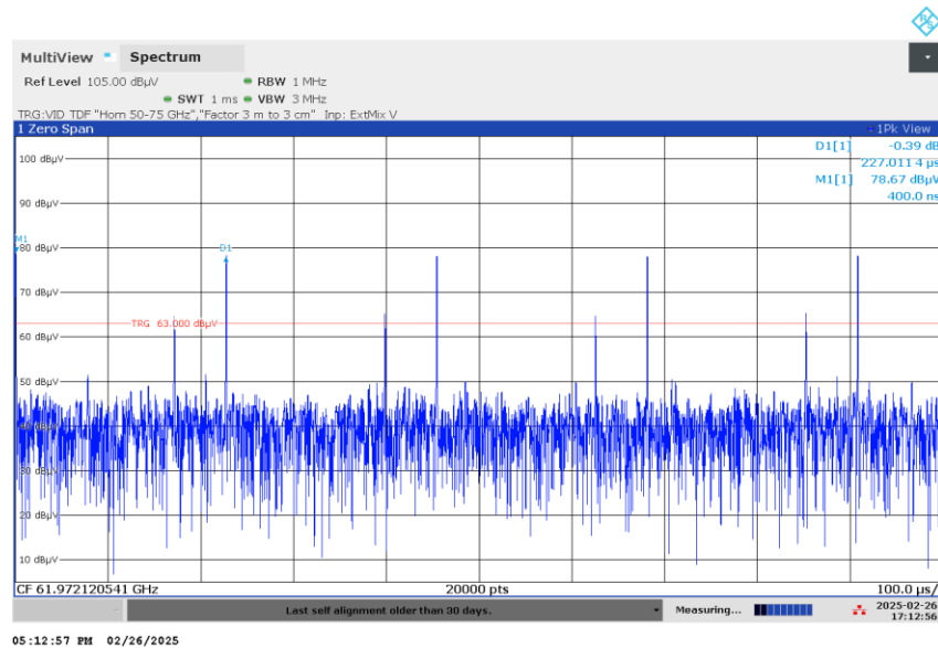
Figure 7.4-3: Field strength of fundamental emissions (Plus timing.), Zero span
