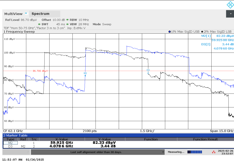
Figure 7.4-2: OBW measurement view
