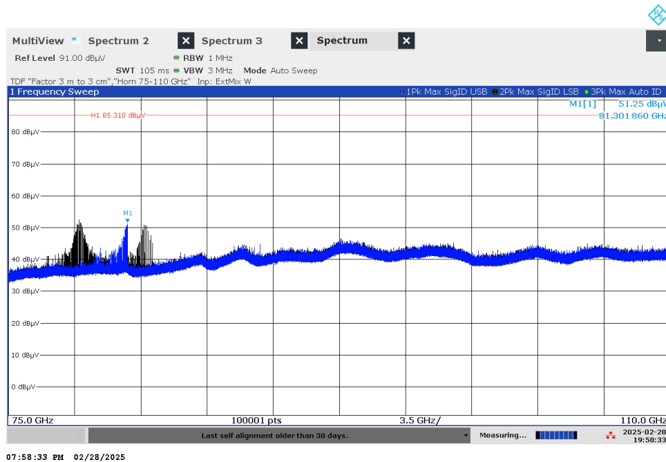
Figure 7.5-6: Radiated spurious emissions 75 GHz-110 GHz
