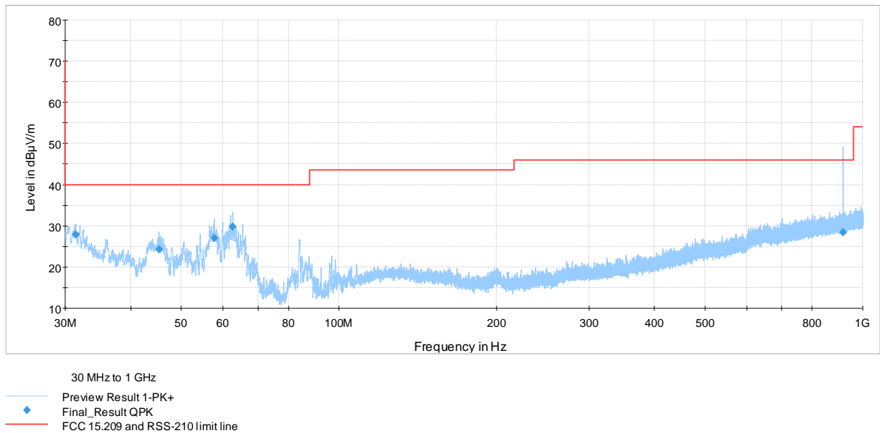
Figure 7.5-1: Radiated spurious emissions below 1000 MHz
