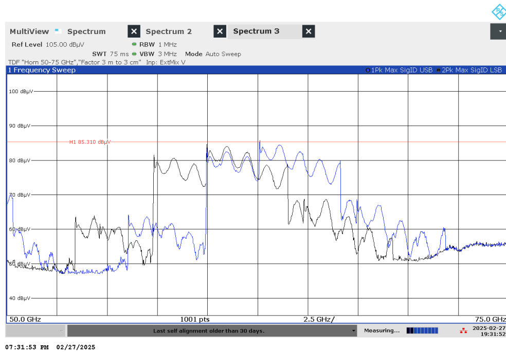
Figure 7.5-5: Radiated spurious emissions 50-75 GHz
