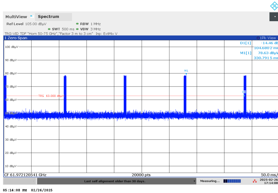
Figure 7.4-4: Field strength of fundamental emissions (Pulse sequences), Zero span
