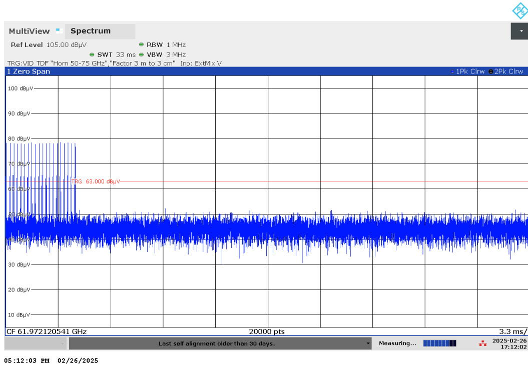
Figure 7.4-5: Off-time duration within 33 ms interval
