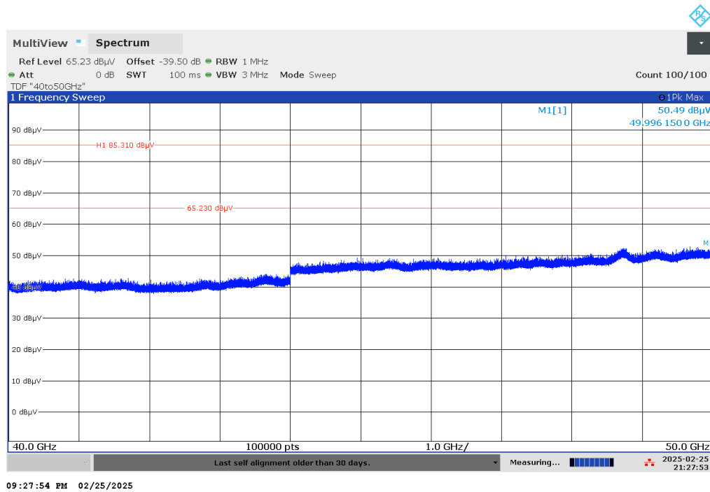
Figure 7.5-4: Radiated spurious emissions 40-50 GHz
