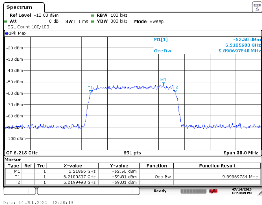
Plot 7-193. AWGN Signal (Demonstration)
