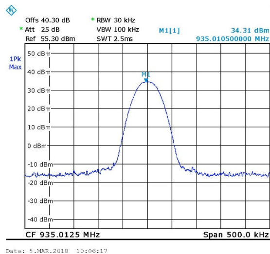
Figure 10. 935.0125MHz, Digital
