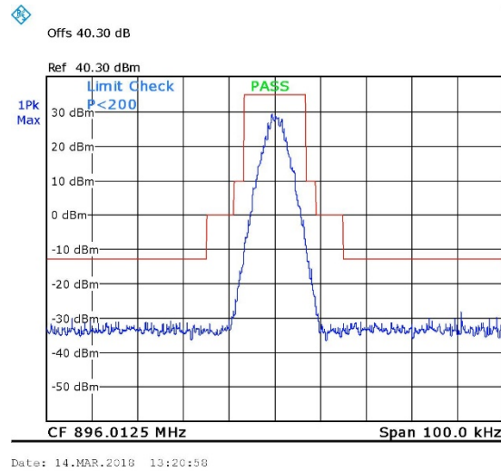
Figure 17. 896.0125MHz, Digital
