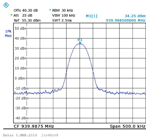
Figure 15. 939.9875MHz, TDMA
