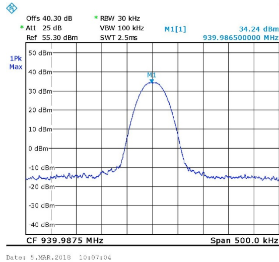
Figure 11. 939.9875MHz, Digital
