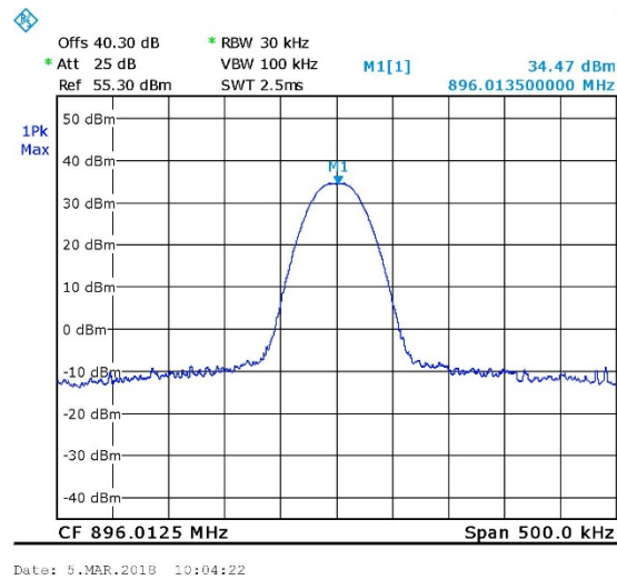
Figure 8. 896.0125MHz, Digital
