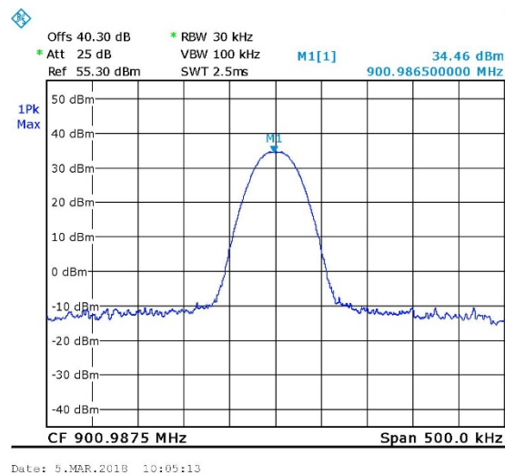
Figure 9. 900.9875MHz, Digital
