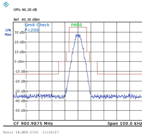
Figure 18. 900.9875MHz, Digital
