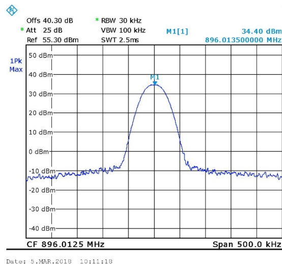
Figure 12. 896.0125MHz, TDMA
