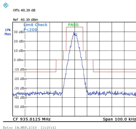
Figure 19. 935.0125MHz, Digital
