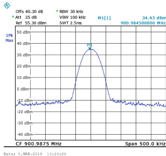
Figure 13. 900.9875MHz, TDMA
