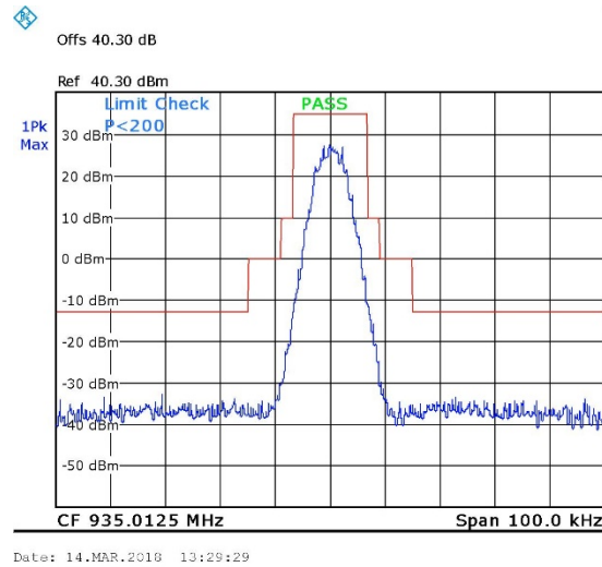
Figure 23. 935.0125MHz, TDMA
