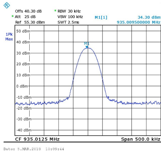
Figure 14. 935.0125MHz, TDMA
