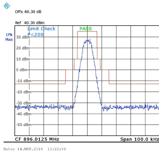
Figure 21. 896.0125MHz, TDMA
