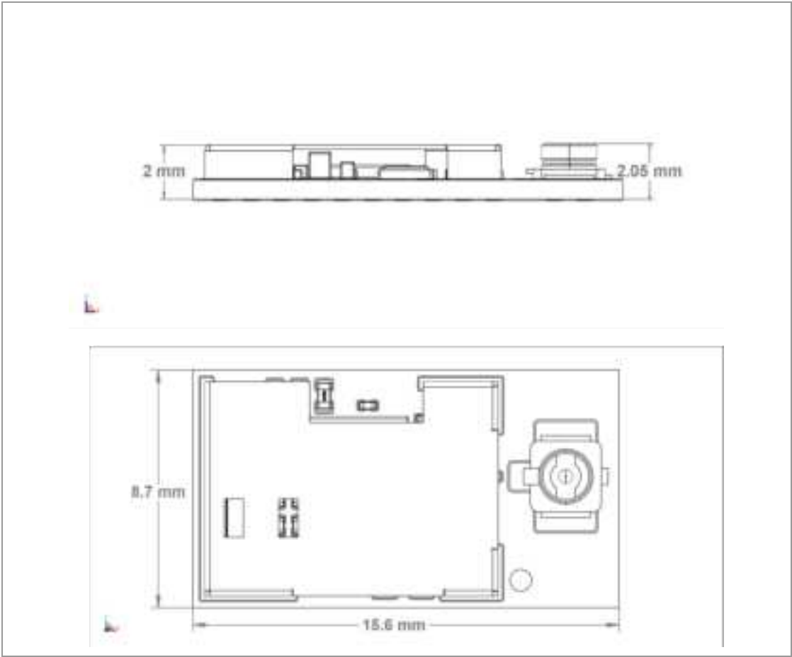
Top View
