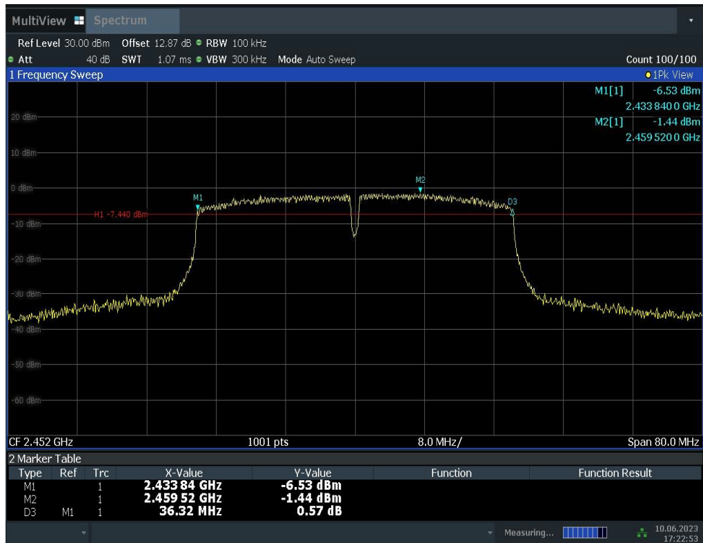
Fig.A.4.12 Occupied 6dB Bandwidth (802.11n-HT40, Ch 9)
