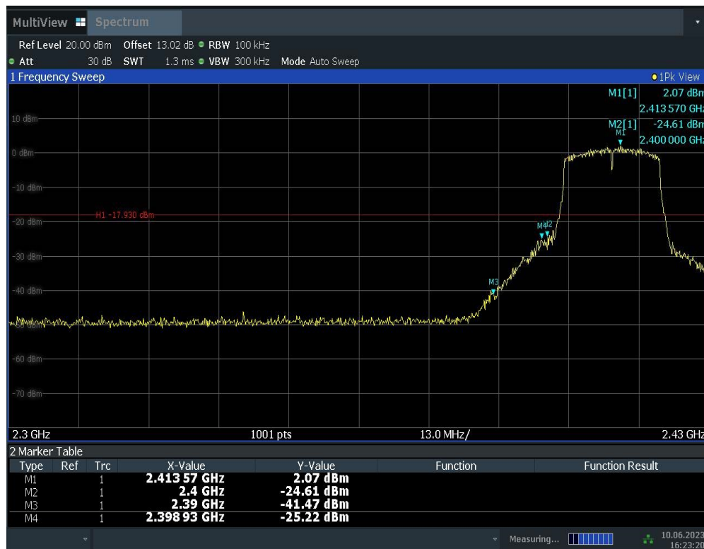
Fig.A.5.5 Band Edges (802.11n-HT20, Ch 1)
