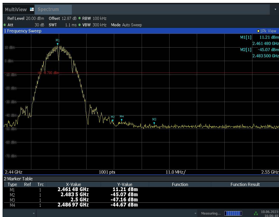
Fig.A.5.2 Band Edges (802.11b, Ch 11)
