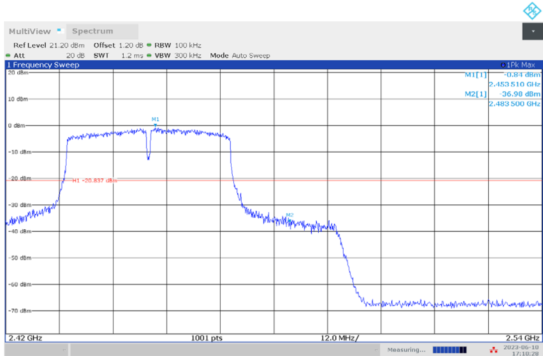
Fig.A.5.8 Band Edges (802.11n-HT40, Ch 9)
