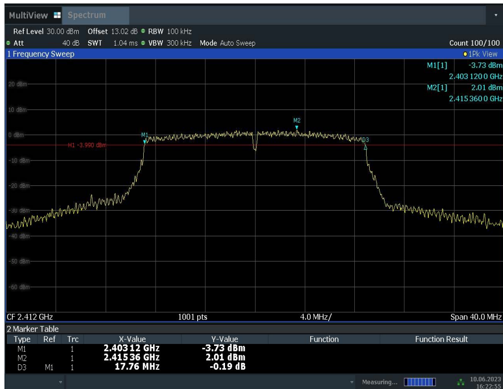
Fig.A.4.7 Occupied 6dB Bandwidth (802.11n-20MHz, Ch 1)
