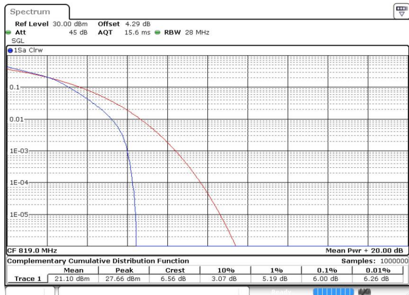
Band26-10MHz-16QAM-26740-50RB#0
