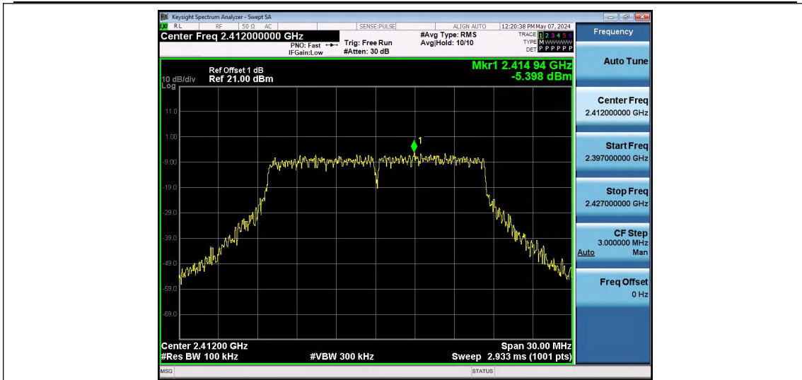
11G-Ant1-2412-0~Reference-PASS
