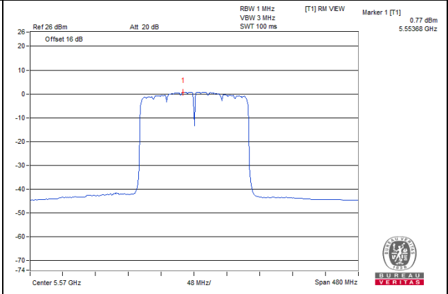
11ax (80MHz) 2S4T TxBF CH114
