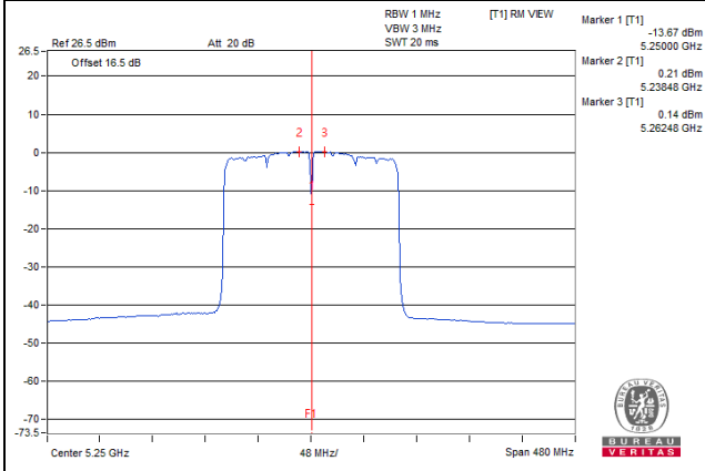
11ax (160MHz) 2S4T TxBF CH50
