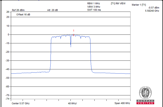
11ax (80MHz) 3S4T TxBF CH114
