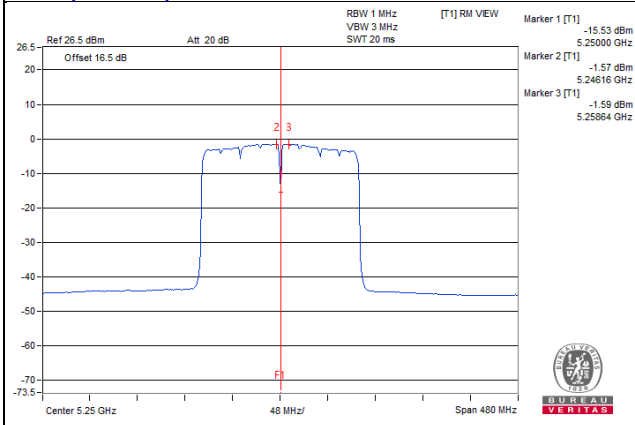
11ax (160MHz) 3S4T TxBF CH50
