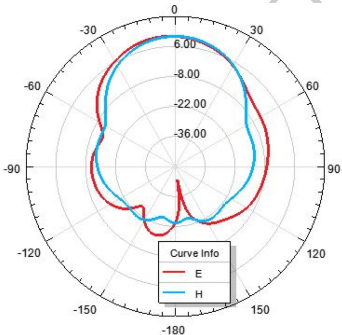
Antenna Radiation Pattern Simulation Data
