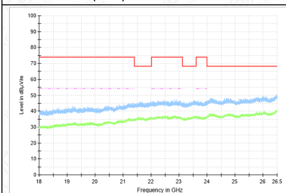
RSE-11AC(80M)-CH155-18GHz-26.5GHz
