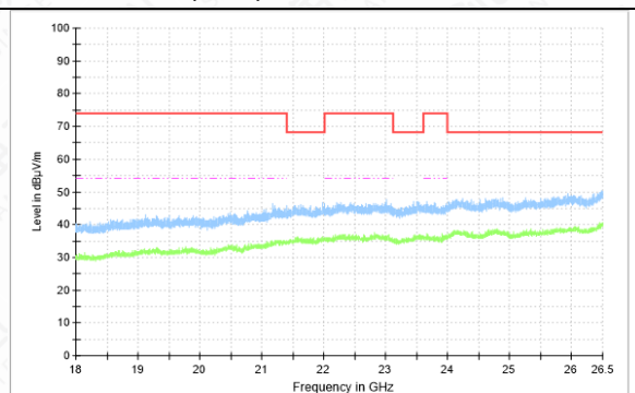
RSE-11N(40M)-CH159-18GHz-26.5GHz
