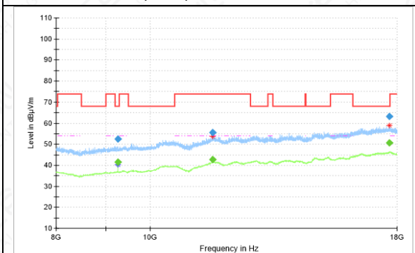
RSE-11N(40M)-CH159-8GHz-18GHz
