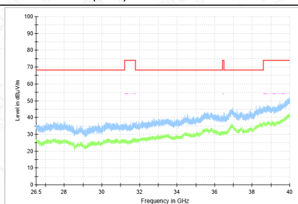
RSE-11AC(80M)-CH155-26.5GHz-40GHz
