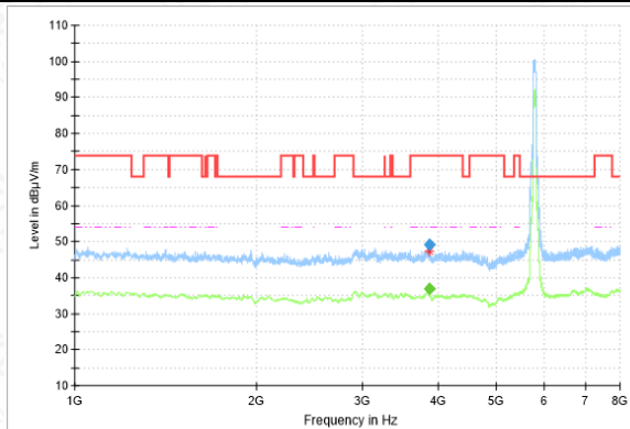
RSE-11AC(80M)-CH155-1GHz-8GHz
