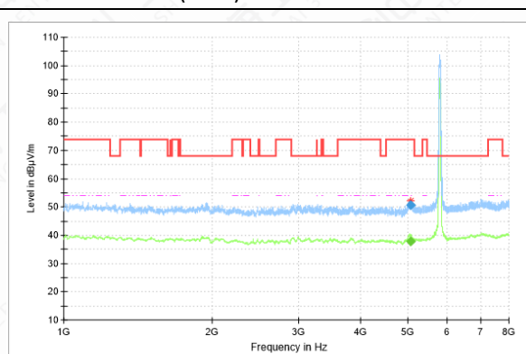
RSE-11N(40M)-CH159-1GHz-8GHz
