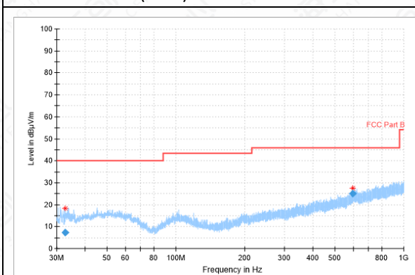
RSE-11N(40M)-CH159-30MHz-1GHz
