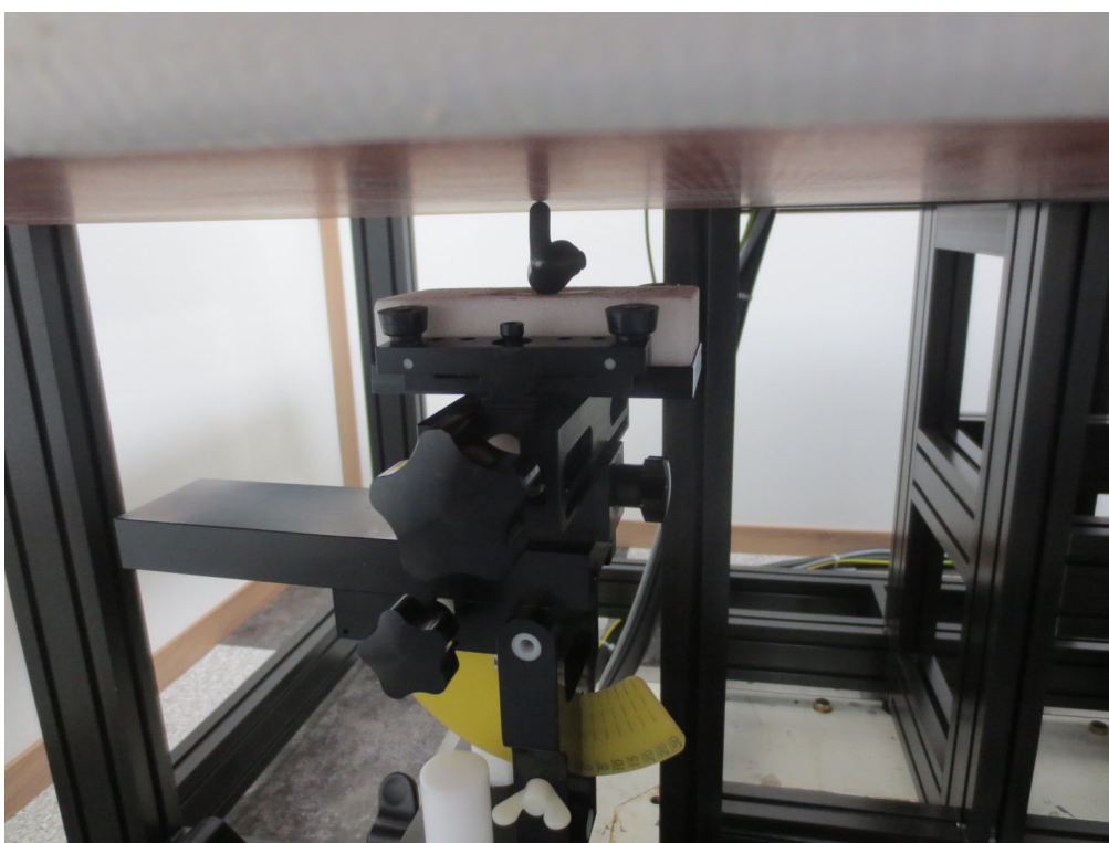
Bottom from Flat Phantom (Separation Distance: 0 cm) – Left Ear
