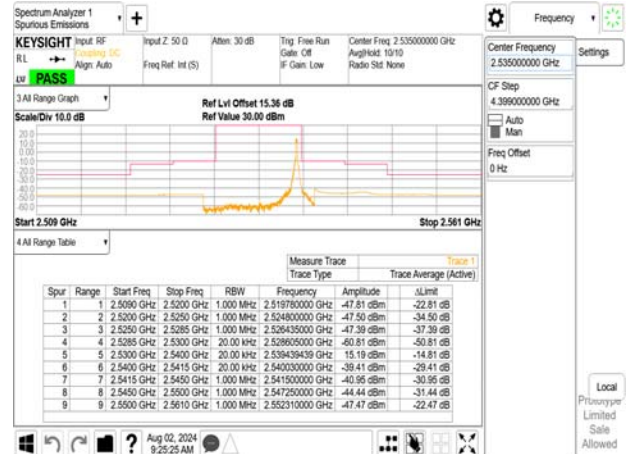
Emission Mask_Band7_10MHz_QPSK_RB1_49_CH21100
