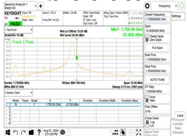
Band Edge_Band4_5MHz_QPSK_RB25_0_CH19975
