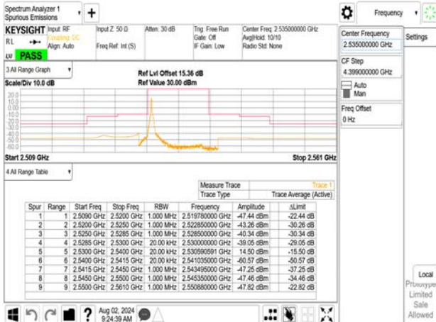
Emission Mask_Band7_10MHz_QPSK_RB1_0_CH21100
