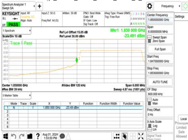
Band Edge_Band2_3MHz_QPSK_RB15_0_CH18185
