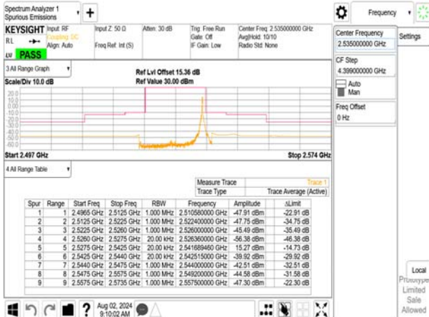
Emission Mask_Band7_15MHz_QPSK_RB1_74_CH21100
