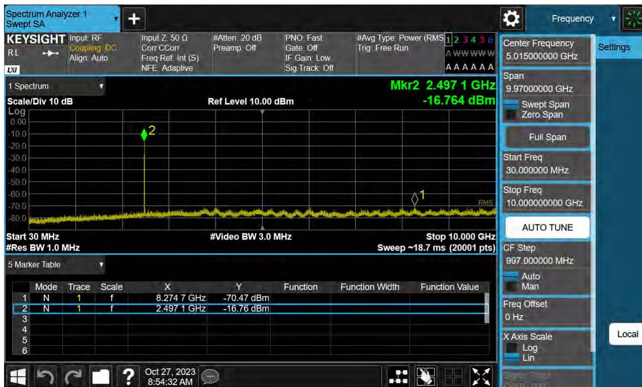
Sub6 n41. Conducted Spurious Plot 1 (15 MHz Ch.500700 BPSK RB 1)
