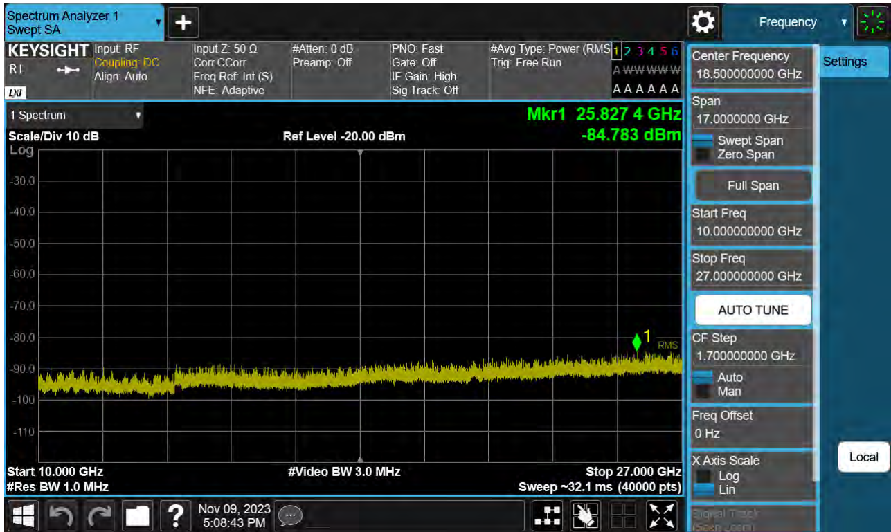
Sub6 n41. Conducted Spurious Plot 2 (25 MHz Ch.535500 BPSK RB 1)
