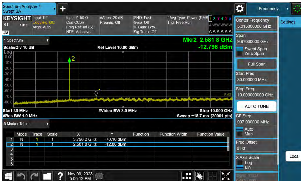
Sub6 n41. Conducted Spurious Plot 1 (25 MHz Ch.518598 BPSK RB 1)
