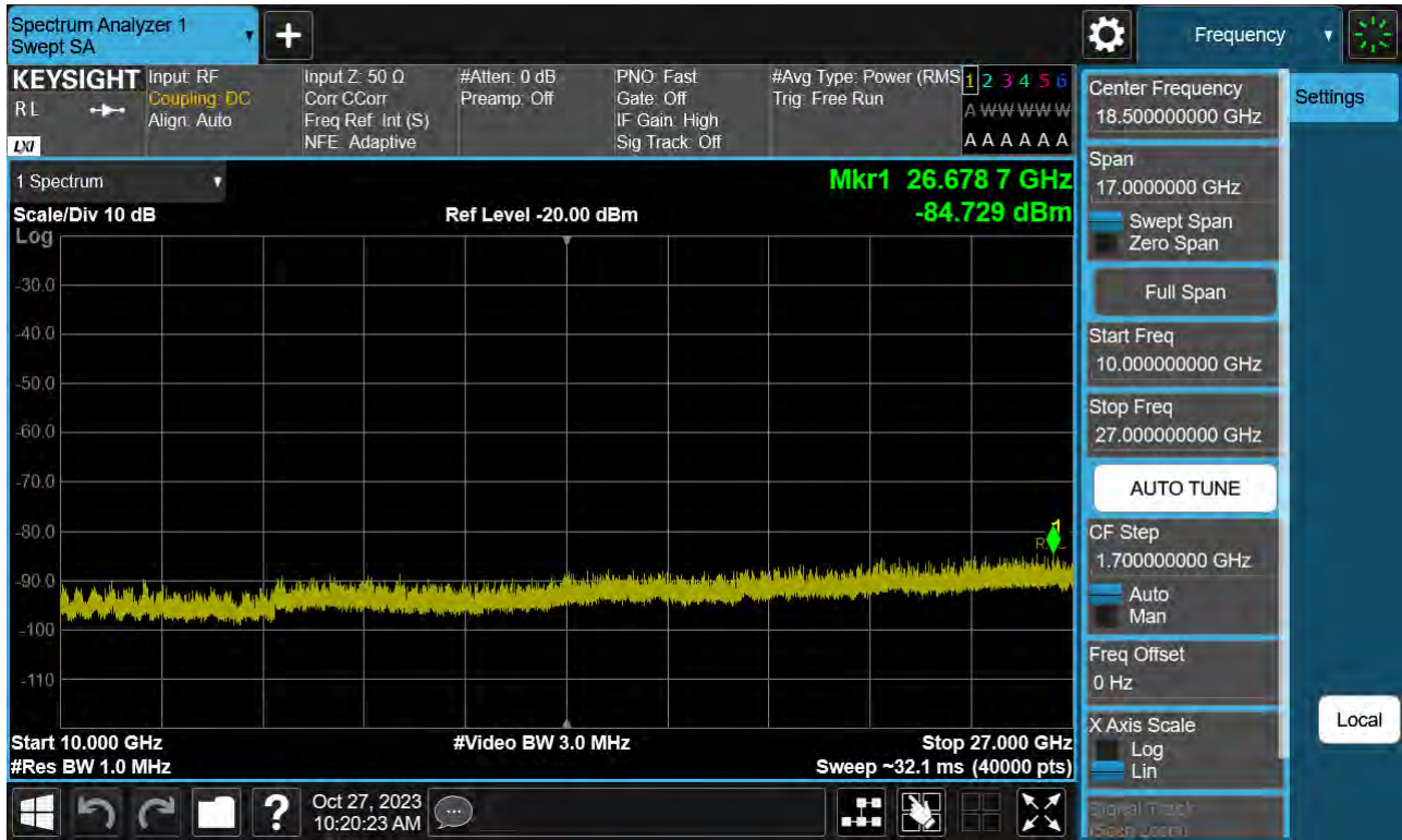
Sub6 n41. Conducted Spurious Plot 2 (70 MHz Ch. 518598 BPSK RB 1)
