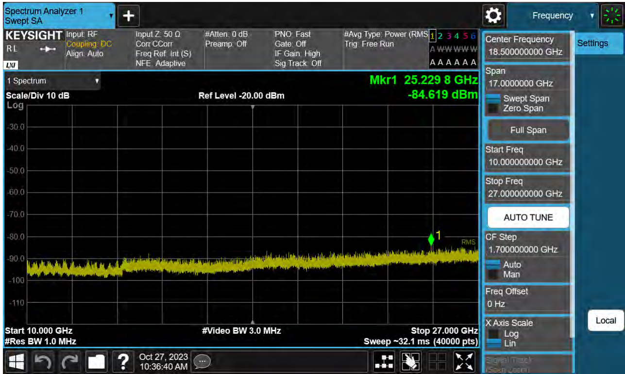
Sub6 n41. Conducted Spurious Plot 2 (80 MHz Ch.529998 BPSK RB 1)
