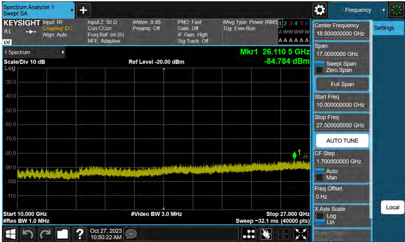
Sub6 n41. Conducted Spurious Plot 2 (90 MHz Ch.528996 BPSK RB 1)
