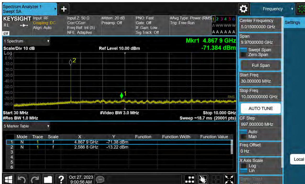
Sub6 n41. Conducted Spurious Plot 1 (15 MHz Ch.518598 BPSK RB 1)
