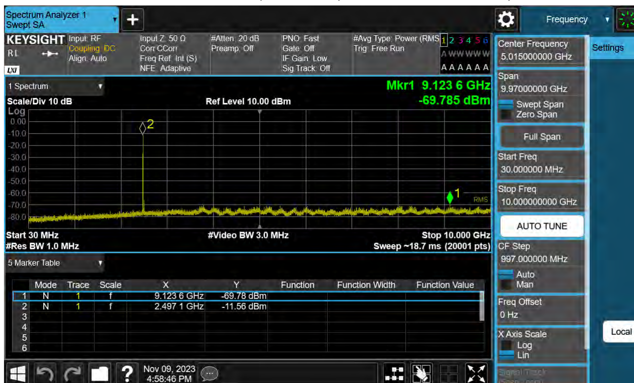
Sub6 n41. Conducted Spurious Plot 1 (25 MHz Ch.501702 BPSK RB 1)
