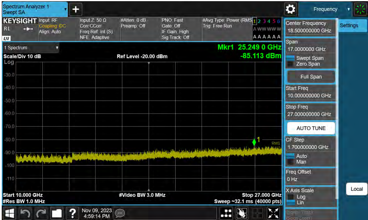
Sub6 n41. Conducted Spurious Plot 2 (25 MHz Ch.501702 BPSK RB 1)
