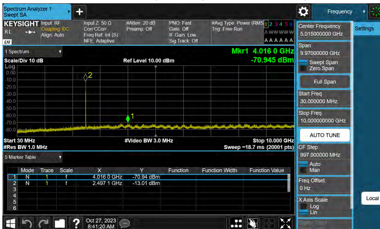
Sub6 n41. Conducted Spurious Plot 1 (10 MHz Ch.500202 BPSK RB 1)
