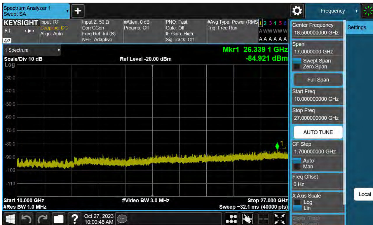
Sub6 n41. Conducted Spurious Plot 2 (60 MHz Ch.505200 BPSK RB 1)
