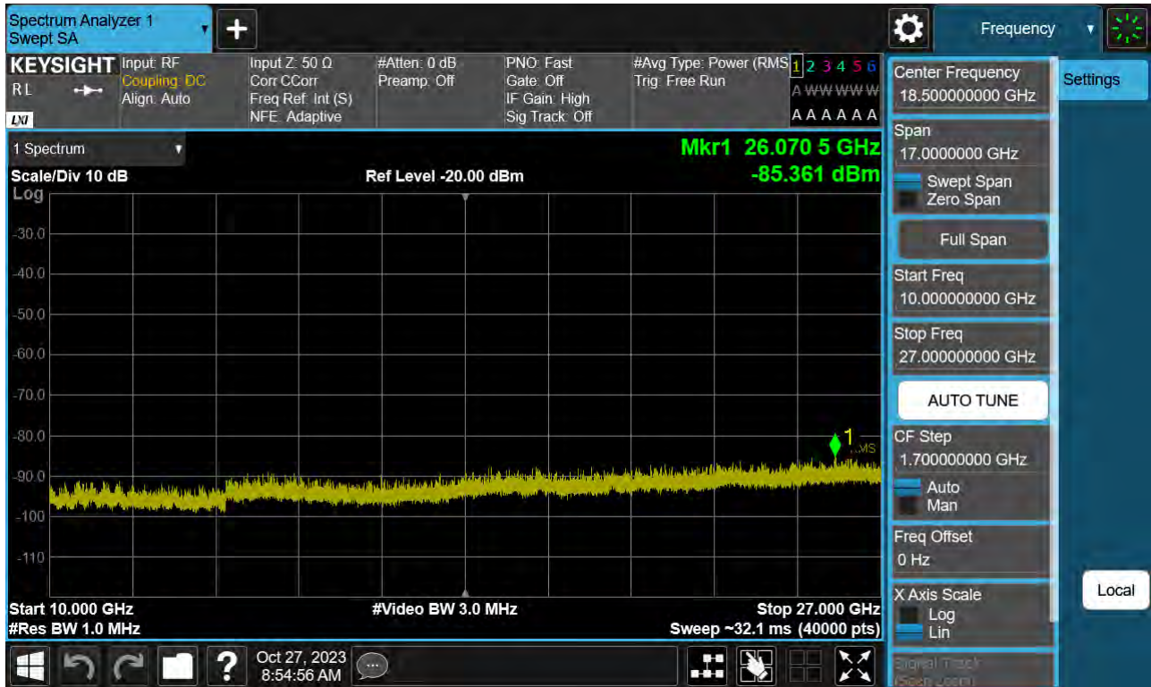
Sub6 n41. Conducted Spurious Plot 2 (15 MHz Ch.500700 BPSK RB 1)
