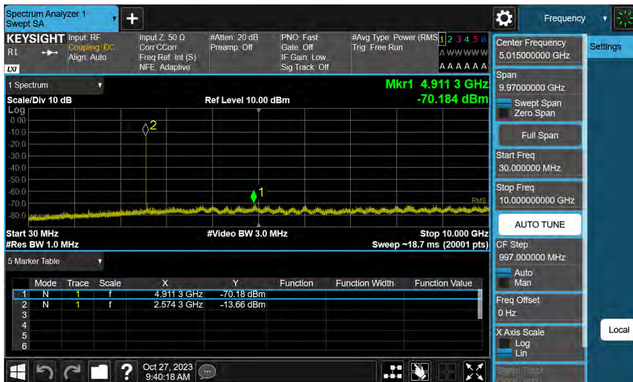
Sub6 n41. Conducted Spurious Plot 1 (40 MHz Ch.518598 BPSK RB 1)
