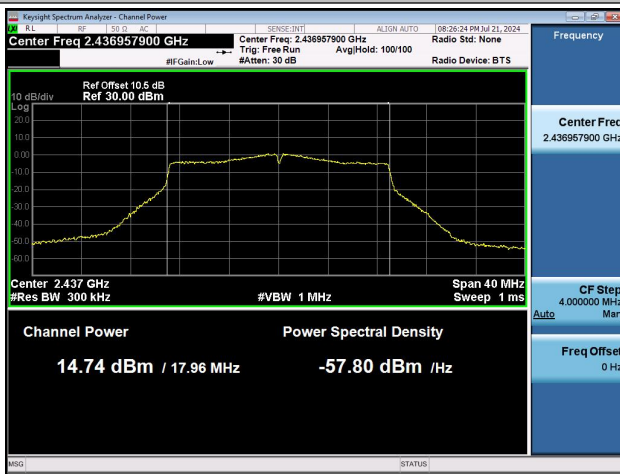
11N20MIMO-Ant0-2437-PASS
