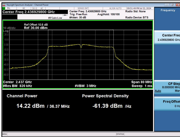
11N40MIMO-Ant1-2437-PASS
