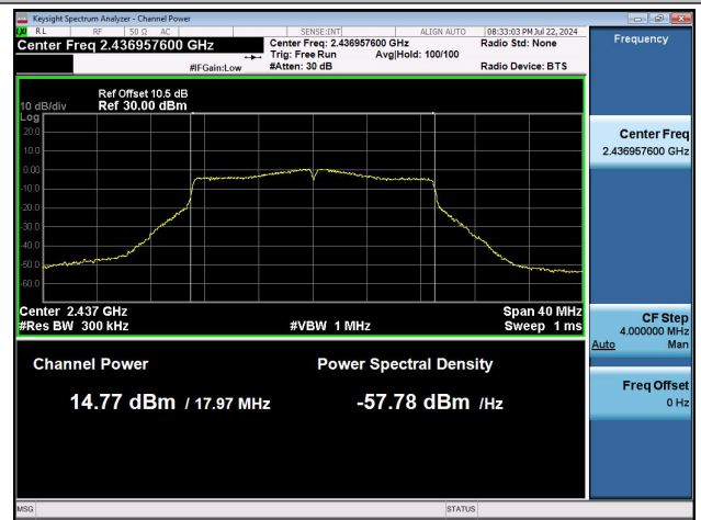
11N20MIMO-Ant1-2437-PASS
