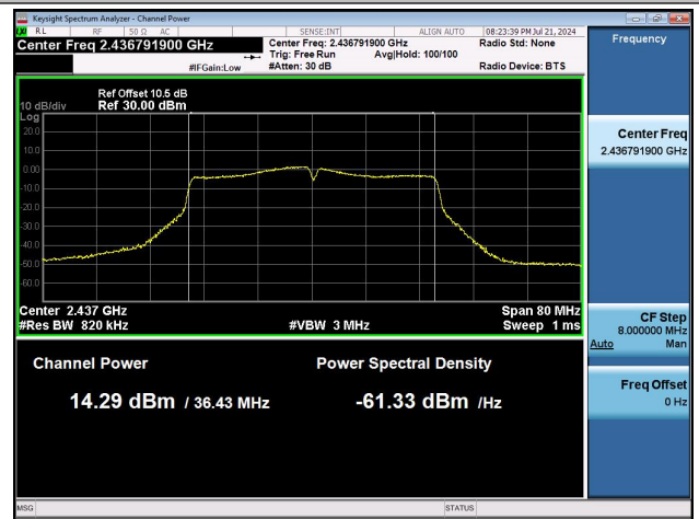
11N40MIMO-Ant0-2437-PASS
