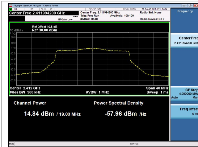
11AX20MIMO-Ant0-2412-PASS
